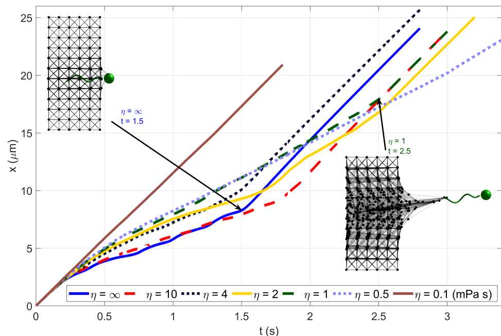
Figure 6. Horizontal position of center of swimmer body as a function of time for a variety of different values of \eta , the dashpot constant. Note that in each case the link stiffness was E = 25 mPa. The insets show snapshots in time of two particular cases.
