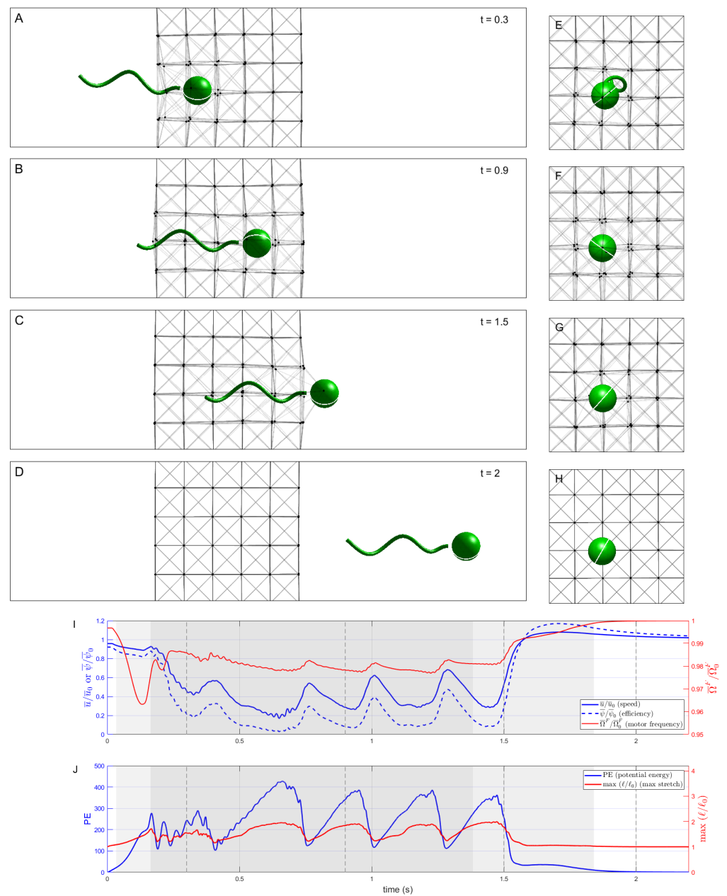
Figure 3. Summary of results for E = 25 mPa, \eta = \infty (Hookean elements). Panels (A–H): side views and frontal views at four selected times, zoomed in to highlight the dynamics near the microswimmer. A white equatorial band is depicted around the cell body to demonstrate rotation. Panel (I): timeseries of swimming speed, motor frequency, and power efficiency, all averaged over a body rotation and normalized to the Newtonian case ( E = 0 mPa). Panel (J): timeseries of potential energy of the network (PE) and the maximum relative strain \ell/\ell_0 . Vertical dashed lines correspond to when each snapshot was taken. Leftmost light gray shading corresponds to when any part of the spherical body but none of the flagellum is inside the rectangular volume initially occupied by the network. Dark shading corresponds to when both the body and flagellum are each at least partially inside. Rightmost light shading corresponds to when part of the flagellum but none of the body is inside. Unshaded sections correspond to when the swimmer is completely outside this rectangular volume. See Supplementary Materials Video S1 for an animated version.
