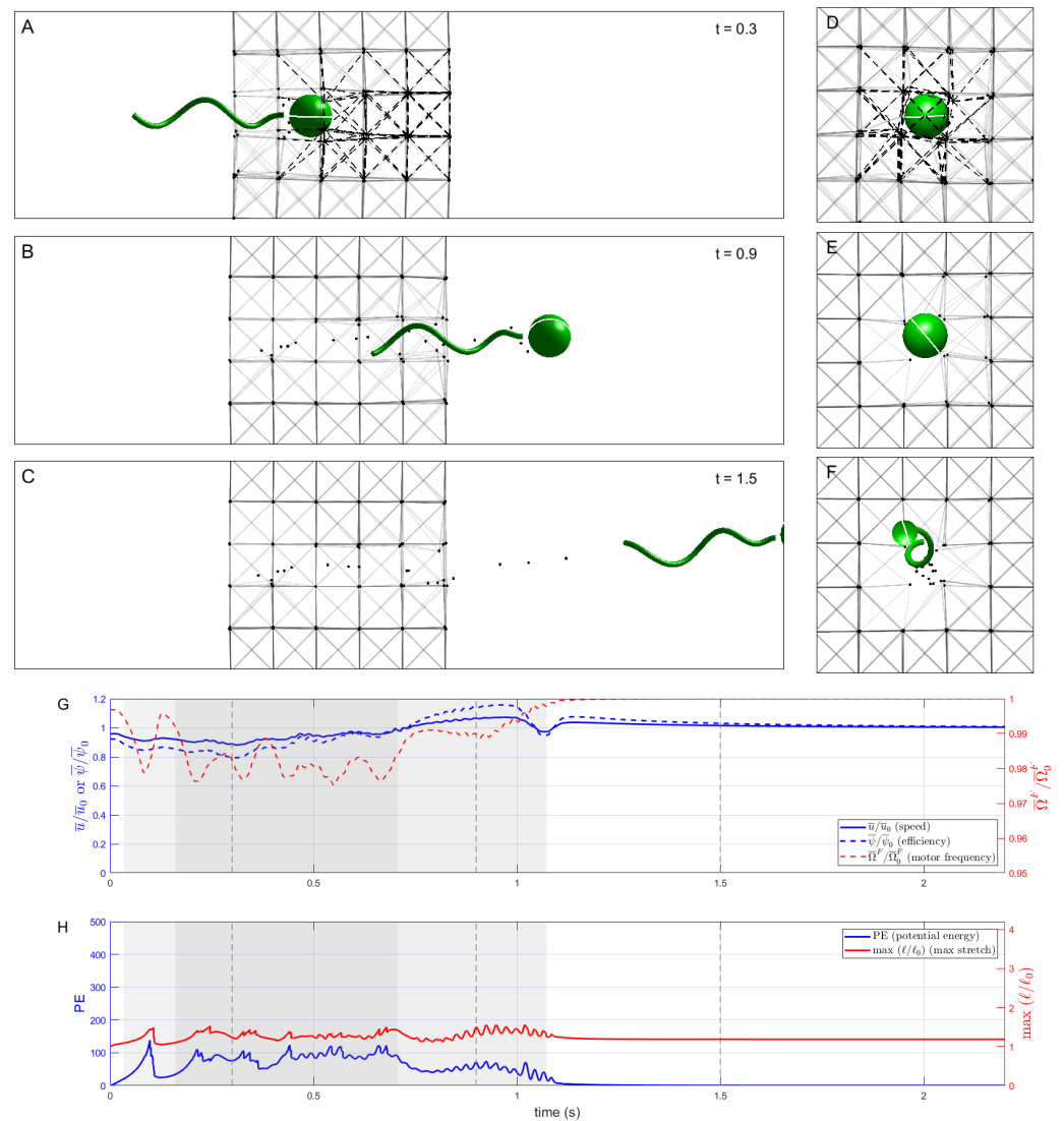
Figure 7. Summary of results for E = 25 mPa, \eta = 10 mPa-s in which network links coming within 0.2R_S of the body surface were permanently destroyed, modeling chemical degradation. See Figure 3 for panel descriptions, but note that panels for t = 2 s are omitted because the swimmer has completely exited the field of view at that time. See in Supplementary Materials Video S4 for an animated version.
