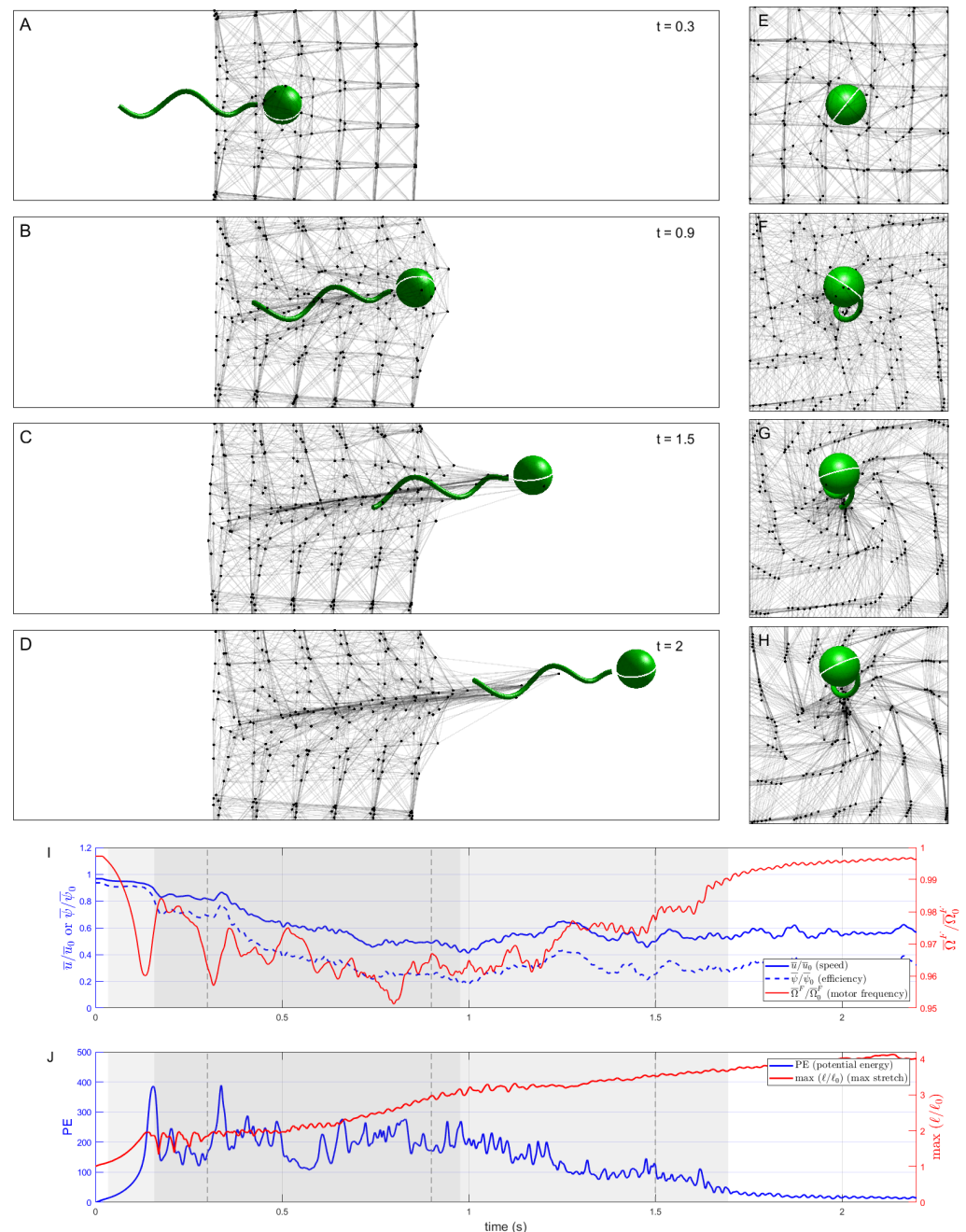
Figure 5. Summary of results for E = 25 mPa, \eta = 1 mPa-s. See Figure 3 for panel descriptions. See in Supplementary Materials Video S3 for an animated version.
