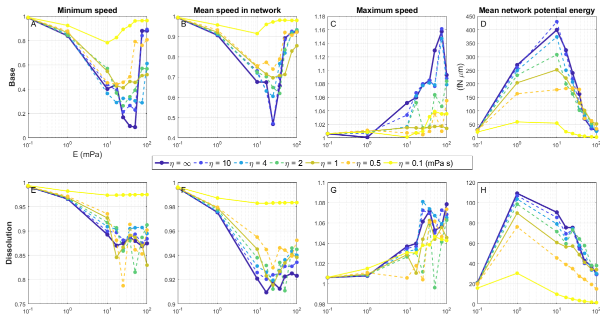
Figure 9. Summary metrics for simulation results across a range of E and \eta , for base case without remodeling (A–D) versus with chemical dissolution (E–H). Minimum and maximum swimming speed over the entire simulation, and mean swimming speed and network potential energy averaged up to the time at which the center of the body reaches the right edge of the network. All speeds are normalized to that of the Newtonian ( E = 0 ) case. Note the different y-axis scales between some base and dissolution panels for clarity.
