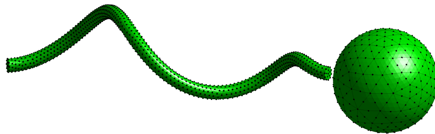
Figure 2. Schematic of the swimming organism used in all examples. It consists of a spherical body and a helical cylindrical flagellum. Note the surface discretization points, which are used in the boundary integration.
