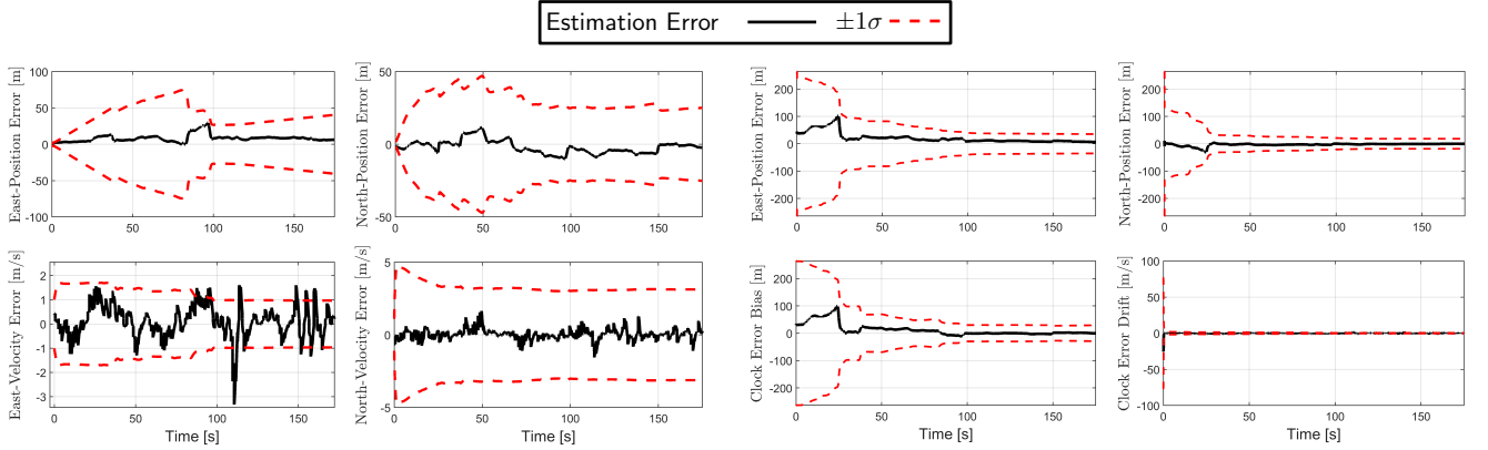
Fig. 4. Radio SLAM base case experimental results showing the estimation error trajectories and corresponding \pm 1\sigma bounds.
