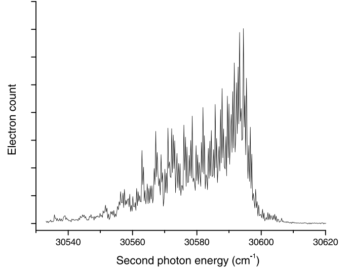
FIG. 7. PFI-ZEKE spectrum of the \text{YbF}^+ X^1\Sigma^+ origin band. The first photon was set to excite the YbF A^2\Pi_{1/2} - X^2\Sigma^+ 0-0 band at 18\,106.3\text{ cm}^{-1} . The high-frequency oscillations of this trace were caused by shot-to-shot amplitude noise.
