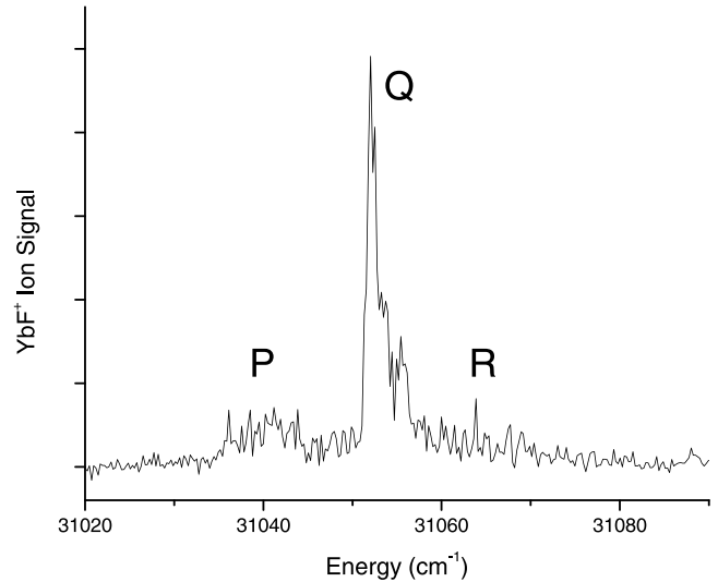
FIG. 2. One-color RE2PI spectrum of the \text{YbF } [31.05]1/2-X^2\Sigma^+ transition. This trace was recorded using detection of the ^{174}\text{YbF}^+ isotopologue.
