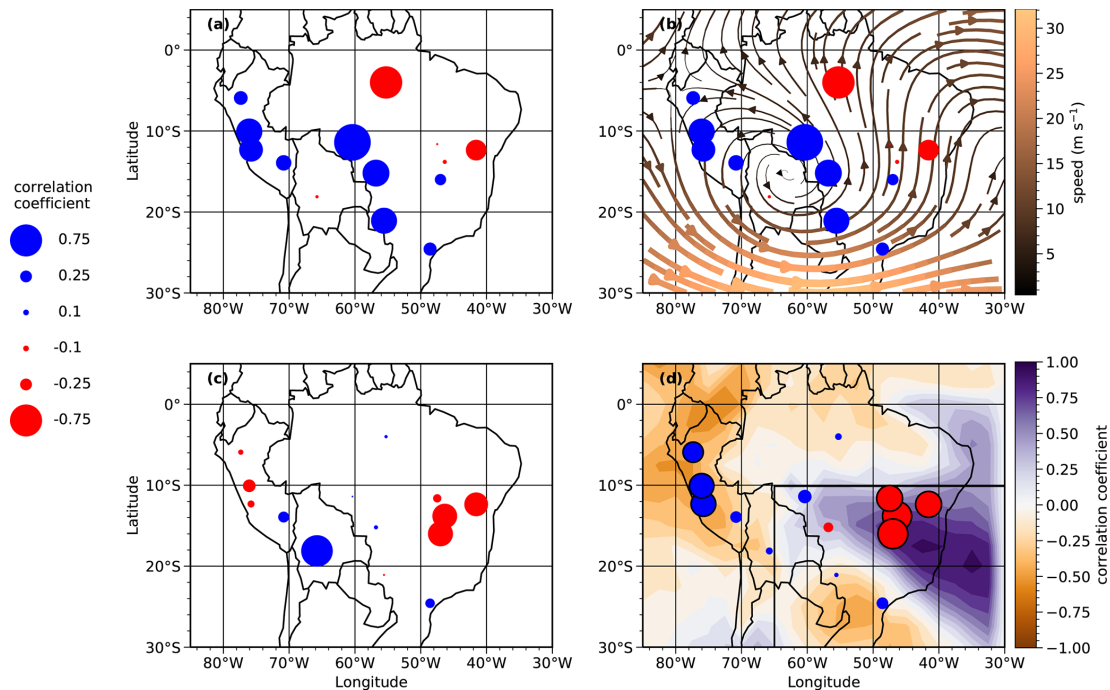
Figure 4. MCEOF patterns and their corresponding dynamic interpretations. (a) MCEOF1 loadings; (b) upper-level (200 hPa) DJF streamlines from ERA5 reanalysis (1979–2019); (c) MCEOF2 loadings; (d) spatial correlation of DJF OLR field with the PC1 of OLR variability derived from the SACZ region (black box). Colored circles indicate the correlation of local precipitation derived from station data with PC1 of the OLR decomposition over the SACZ region.
