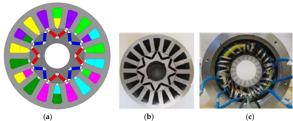
Figure 6. The 6-phase 18-slot/8-pole machine: (a) schematic with winding layout and top view of the motor, (b) without copper coil and PM, and (c) with copper coil and others [4]. ©IEEE. Reprinted with permission from Patel, V.; Wang, J.; Wang, W.; Chen, X. The 6-phase fractional-slot-per-pole-phase permanent-magnet machines with low space harmonics electric vehicle application. IEEE Transactions on Industry Application, vol. 50, no. 4, July 2014.
