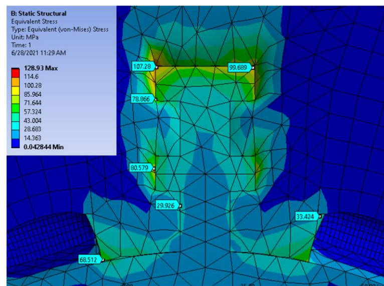
Figure 15. Mechanical analysis of the proposed 6Φ-S-FSCW-Fer-SPMSM at 3750 rpm.
