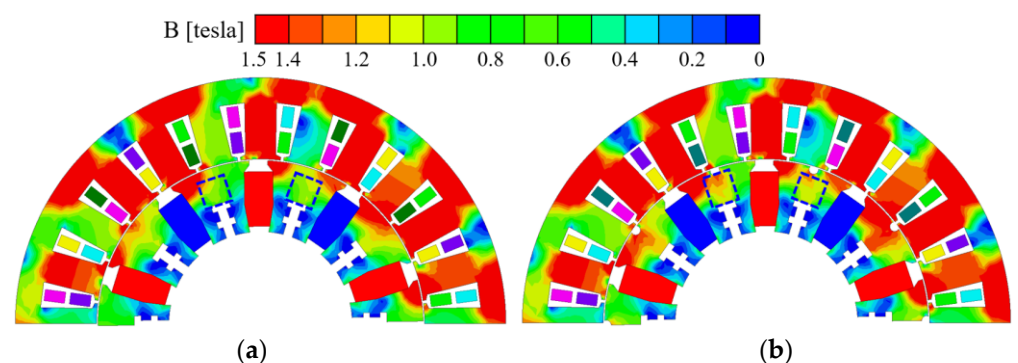
Figure 11. Flux density distribution of 6 \Phi -SS-FSCW-Fer-SIPMSM with (a) shaft only and (b) shaft and circular notch on the rotor.
