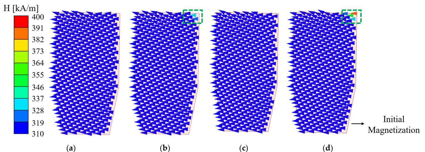
Figure 18. Magnetic field ( H ) distribution of 6Φ-SS-FSCW-Fer-SIPMSM at -40 °C when the motor current was (a) 2.6\times and (b) 2.8\times rated current, and 80 °C when the motor current was (c) 2.6\times and (d) 3.4\times rated current.
