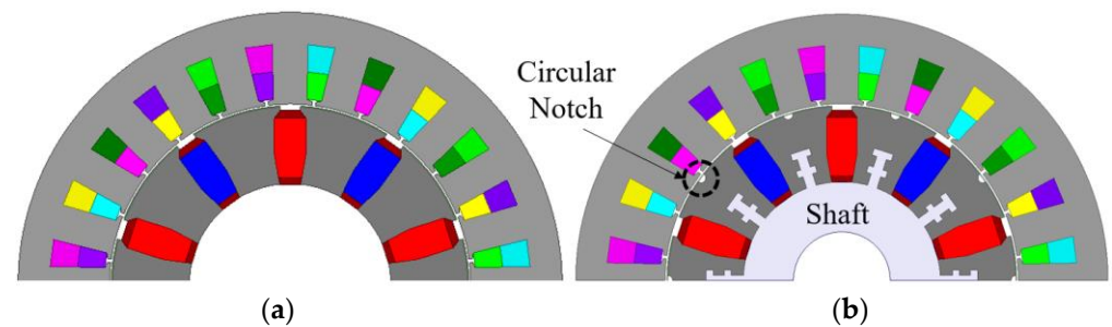
Figure 10. Design of 6 \Phi -SS-FSCW-Fer-SIPMSM (a) without and (b) with circular notch on the rotor and rectangular nonmagnetic shaft fixture.
