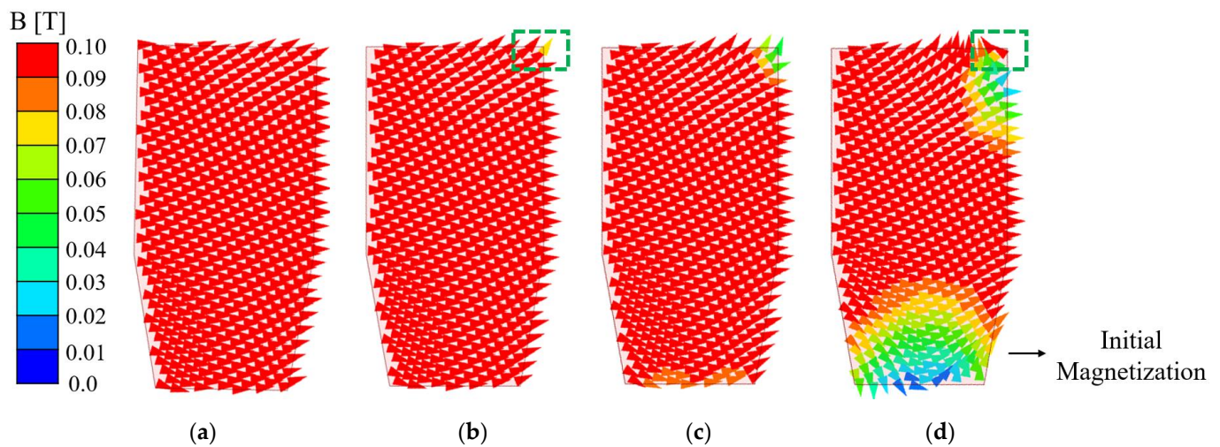
Figure 17. Flux density ( B ) distribution of 6Φ-SS-FSCW-Fer-SIPMSM at -40 °C when the motor current was (a) 2.6\times and (b) 2.8\times rated current, and 80 °C when the motor current was (c) 2.6\times and (d) 3.4\times rated current.
