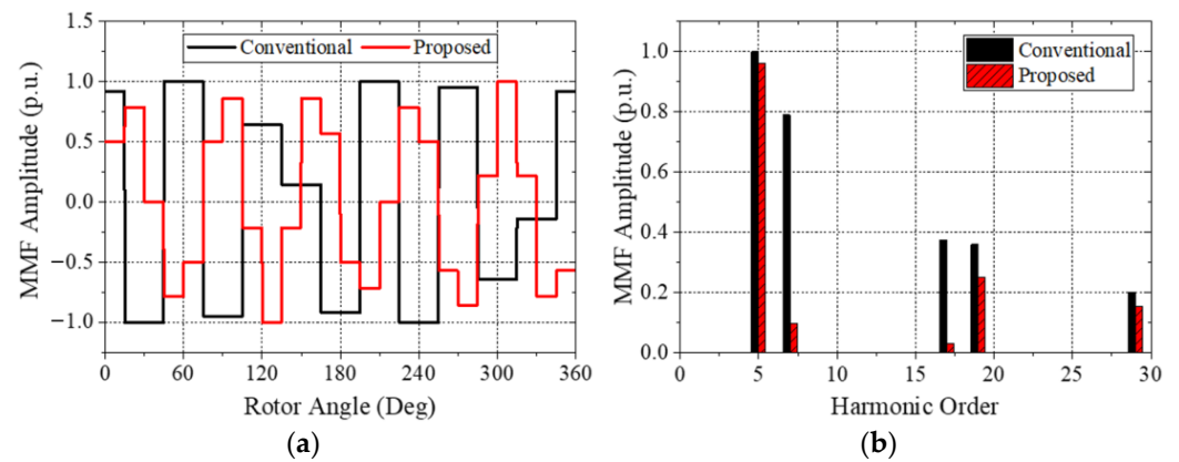
Figure 5. Total MMF distribution (a) profile and (b) harmonic spectrum of the conventional and proposed FSCW motor.
