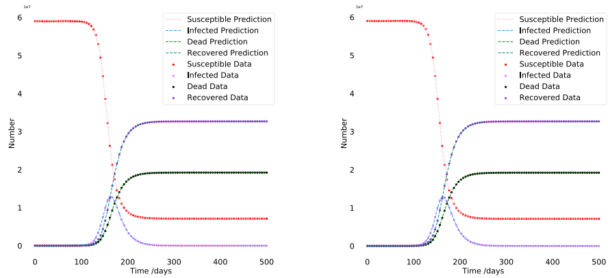
Figure 8: 100000% search range for NN Output (Left) vs LSODA generation from Learnable Parameters (Right).
