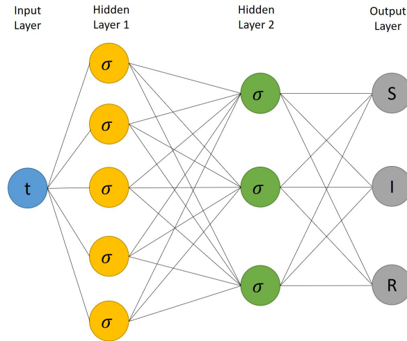
Figure 3: A Simple DINNs Architecture (input: time, has a size of 1 and the output can vary in size (S,I,R)).
