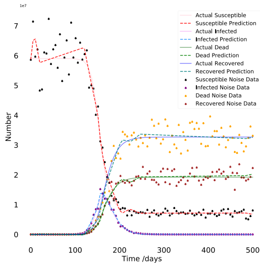
(c) 10% – Neural Network's System.
