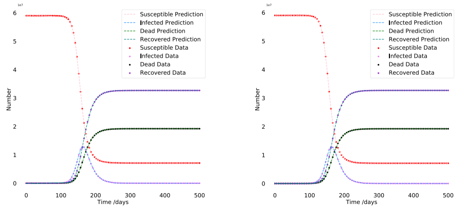
Figure 7: 10000% search range for NN Output (Left) vs LSODA generation from Learnable Parameters (Right).
