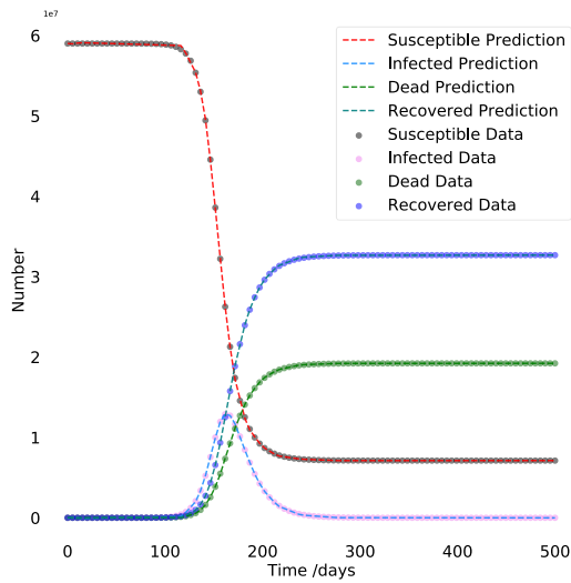
(c) 100 points – Neural Network's System.
