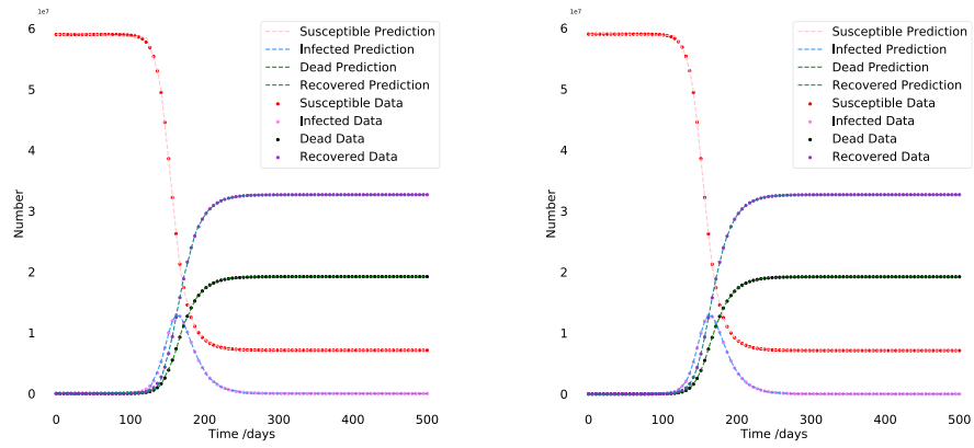
Figure 6: 1000% search range for NN Output (Left) vs LSODA generation from Learnable Parameters (Right).
