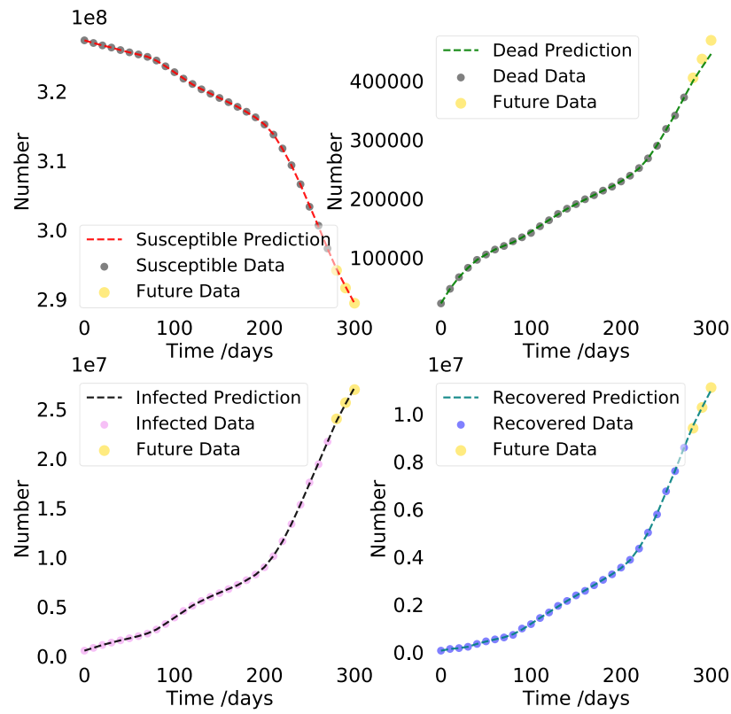
Figure 13: DINN's output on COVID real-life cumulative cases over 310 days.
