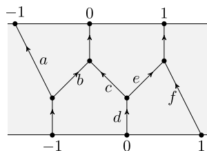
Fig. 3. A network.
