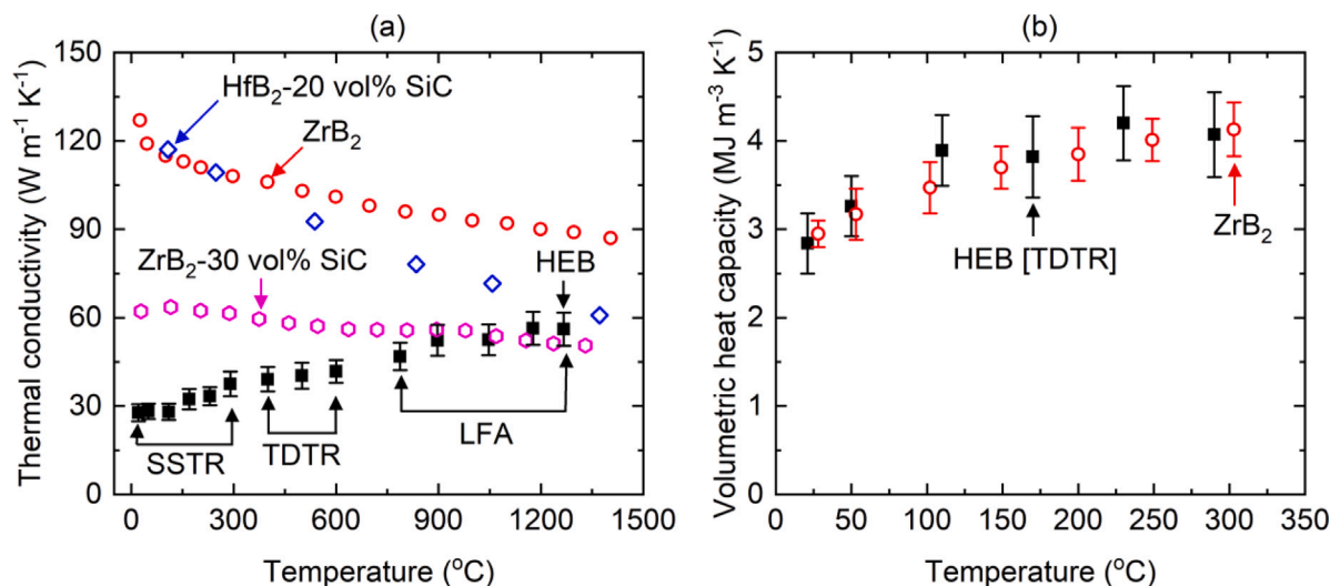
Fig. 2. (a) Temperature-dependent thermal conductivity of HEB measured via three different techniques: SSTR (21–290 ^{\circ}\text{C} ), TDTR (400–600 ^{\circ}\text{C} ), and LFA (787–1267 ^{\circ}\text{C} ). For comparison, we also include the thermal conductivity of ZrB 2 [37], ZrB 2 -30 vol% SiC [55], and HfB 2 -20 vol% SiC [60] from literature. (b) Temperature-dependent heat capacity of HEB along with that of ZrB 2 [37].
