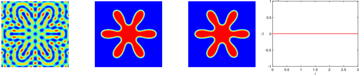
Fig. 5. Example 2B. Profiles of \phi at T = 0.1 . Dynamics driven by the Cahn-Hilliard equation using GSAV/BDF2 scheme (first), R-GSAV/BDF2 scheme (second) and reference solution (third), and the evolution of \zeta_0^{n+1} (fourth).
