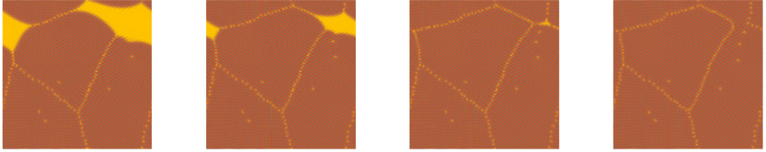
(c) profiles of \phi at T = 800, 900, 1000, 2000
