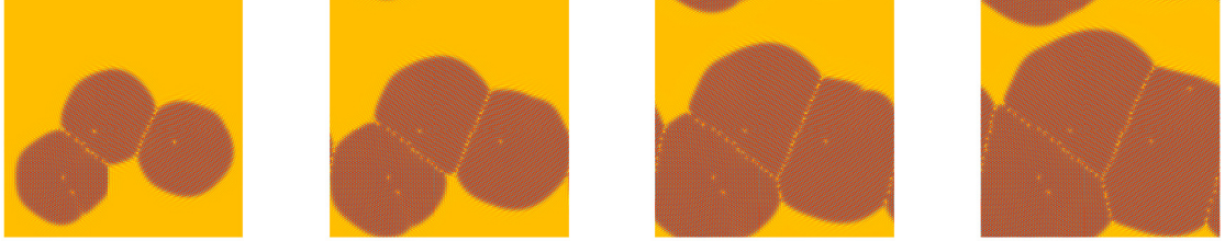
(b) profiles of \phi at T = 400, 500, 600, 700
