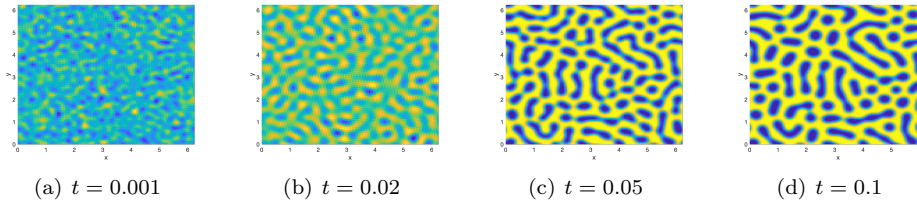
FIG. 6. Numerical solutions of the Cahn–Hilliard equation at t = 0.001, 0.02, 0.05, 0.1 computed by the scheme (5.9)–(5.10).
