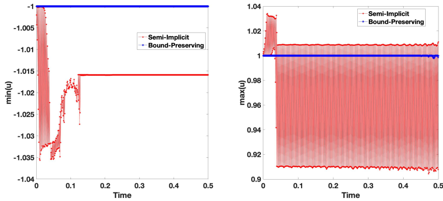
FIG. 3. Evolution of \max\{u\} and \min\{u\} with respect to time for the semi-implicit scheme (6.3) and the bound preserving scheme (5.4)–(5.5).
