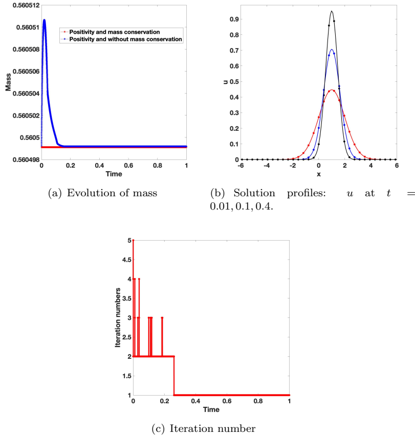
FIG. 8. (a): Evolution of mass by (5.14)–(5.15) and (5.16)–(5.17). (b): Solution profiles by (5.16)–(5.17). (c): Iteration numbers for solving \xi^{n+1} at each time step of (5.16)–(5.17).
