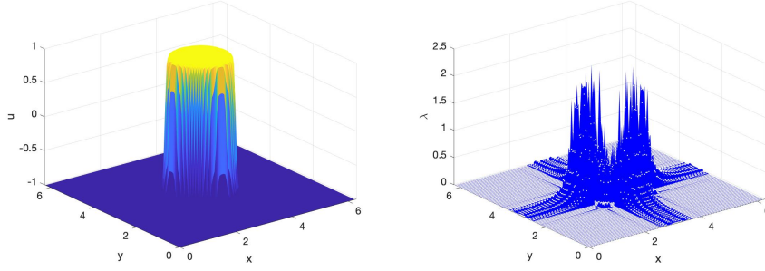
FIG. 1. Numerical solution u and Lagrange multiplier \lambda at T = 0.001 computed by scheme (2.5)–(2.6) with k = 2 and \delta t = 10^{-6} .
