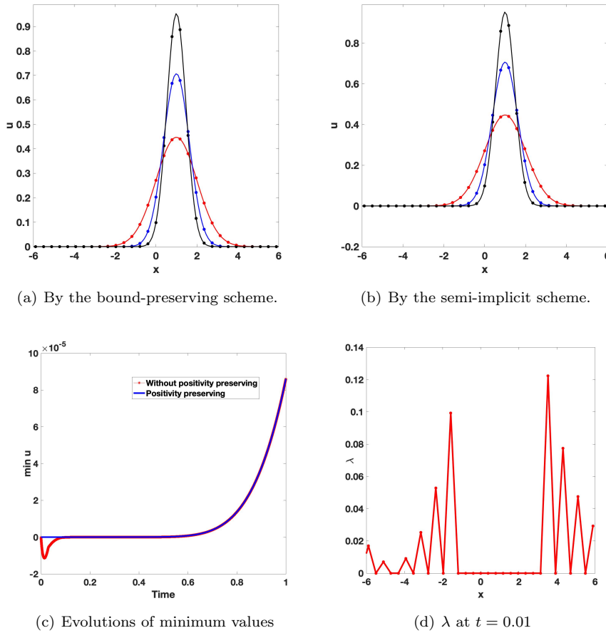
FIG. 7. (a)–(b): Numerical solutions computed with 32 Fourier modes plotted on the 256 uniform grids using (5.14)–(5.15) and (6.10). (c): Evolutions of minimal values using (5.14)–(5.15) and (6.10). (d): Lagrange multiplier \lambda at t = 0.01 using (5.14)–(5.15).
