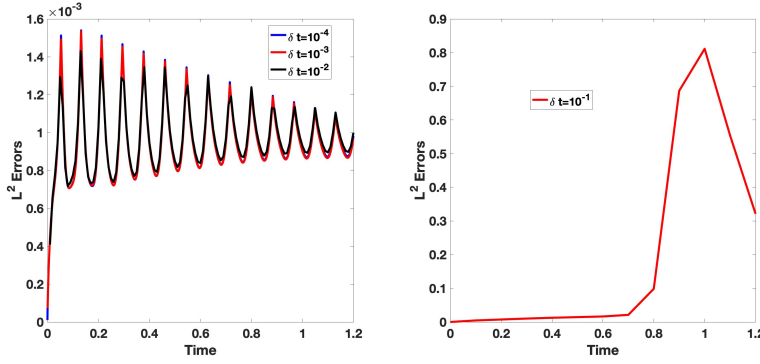
FIG. 4. L^2 errors with different time steps for porous medium equation (6.4) using a second-order bound preserving scheme.
