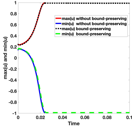
FIG. 5. The evolution of \max_{i,j} u_{i,j}^n and \min_{i,j} u_{i,j}^n with respect to time computed by the scheme (6.9) up to t \approx .025 and by the scheme (5.9)–(5.10) up to t = 0.1 .
