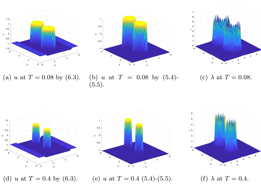
FIG. 2. (a) and (d): Numerical solutions at T = 0.08, 0.4 computed by (6.3). (b)–(c) and (e)–(f): numerical solutions and Lagrange multiplier \lambda at T = 0.08, 0.4 computed by (5.4)–(5.5).
