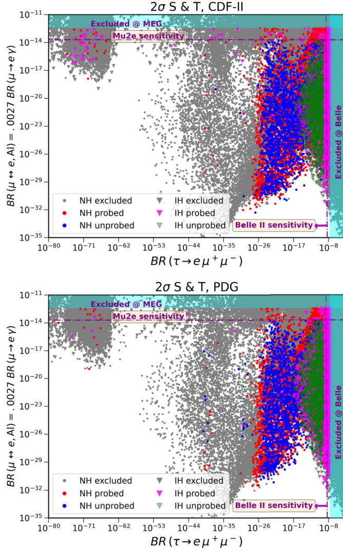
Fig. 3. LFV observables \tau \rightarrow e\mu^+\mu^- and \mu \rightarrow e\gamma for normal ( \bullet ) and inverted ordering ( \blacktriangledown ). All points explain (g-2)_\mu ; in the top plot, we also explain the CDF anomaly, while we ignore CDF in the bottom plot. Gray data points are excluded by the current experimental bounds listed in Table 1. Red/pink data points can be probed in future experiments. Blue/green points cannot be probed in future experiments. Cyan colored band (dashed purple line) is the current exclusion (future sensitivity) limit for \tau \rightarrow e\mu^+\mu^- and \mu \rightarrow e\gamma .
