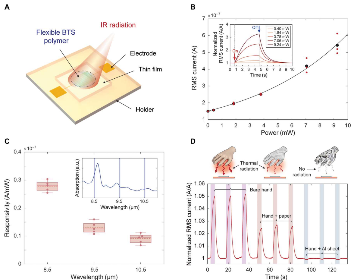
Fig. 5. IR sensor based on flexible BTS polymer. (A) Schematic of the fabricated long-wave, thermal IR detector. (B) Current as a function of IR power irradiated at a wavelength of 8.5 \mu\text{m} . Inset: Representative current profile during a 4-s period of IR exposure in air with different power. Current is measured using an applied voltage of 1 V at 200 Hz. (C) Responsivity of the IR detector at different wavelengths. Inset: Wavelength-dependent absorption intensity of the block copolymer. (D) Real-time detection of thermal radiation generated by a hand wave motion. Covering the hand with a sheet of paper, the rise in current is reduced due to limited transmission of irradiation power. Covering the hand with an aluminum sheet, no change or decrease in current is observed due to IR reflection.
