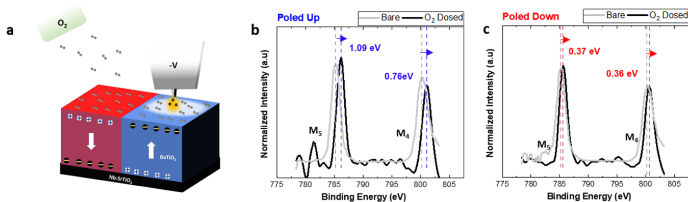
Figure 3. Effect of O 2 adsorption on the Ba M XAS spectra. (a) Schematic of O 2 dosing experiment on pre-poled areas on the sample. (b) Comparison of Ba M XAS spectra on bare and O 2 dosed surfaces with upward polarization and (c) downward polarization.
