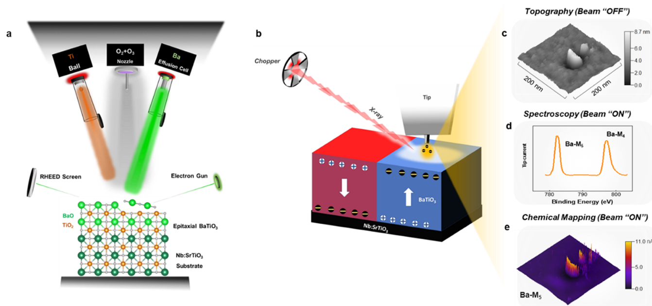
Figure 1. Introduction to the MBE synthesis method and SX-STM technique. (a) Schematic of MBE chamber with a Ti ball source, Ba Knudsen effusion cells, and O 2 /O 3 source during the growth of a BaO monolayer on the surface of epitaxial BaTiO 3 on the Nb:SrTiO 3 substrate. Ba, Ti, Sr, and O atoms are shown in light green, orange, dark green, and gray, respectively. (b) Schematic of a polarized BaTiO 3 film tunneling photoelectrons to the STM tip in near-field mode. (c) Schematic of a three-dimensional (3D) topographical map obtained in the beam “OFF” mode. (d) Schematic of XAS spectra obtained from the point of interest in spectroscopy mode. (e) Schematic of an elemental map obtained in the beam “ON” mode from the same area resolving surface chemistry.
