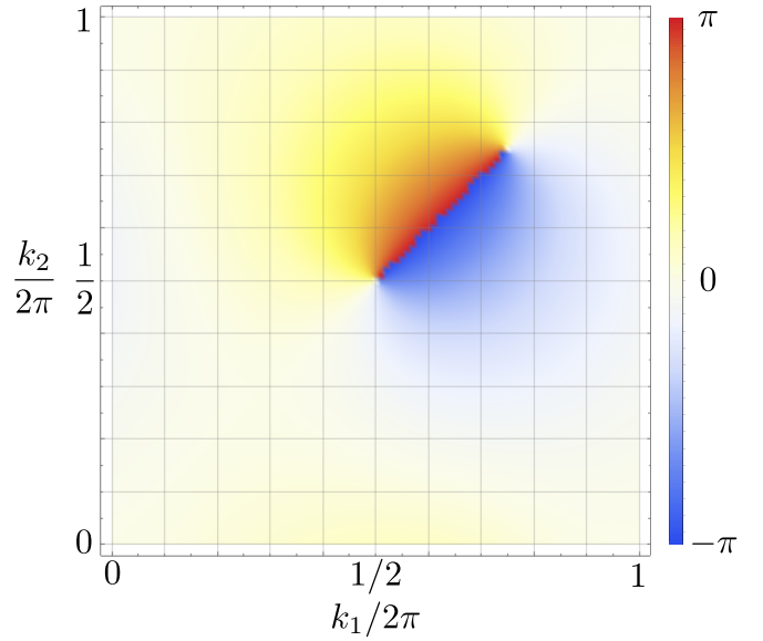
FIG. 3. Phase \xi_{\mathbf{q}}(\mathbf{k}) in Eq. (44) for \mathbf{q} = \frac{\pi}{2}\mathbf{b}_1 + \frac{\pi}{2}\mathbf{b}_2 , plotted as a density. Note the branch cut linking (1/2, 1/2) to (3/4, 3/4) .
