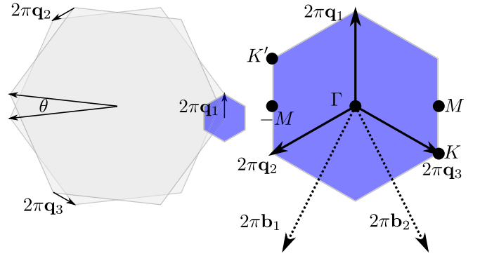
FIG. 4. Construction and conventions of the moiré BZ, blue hexagon, from the graphene layers with relative twist \theta .
