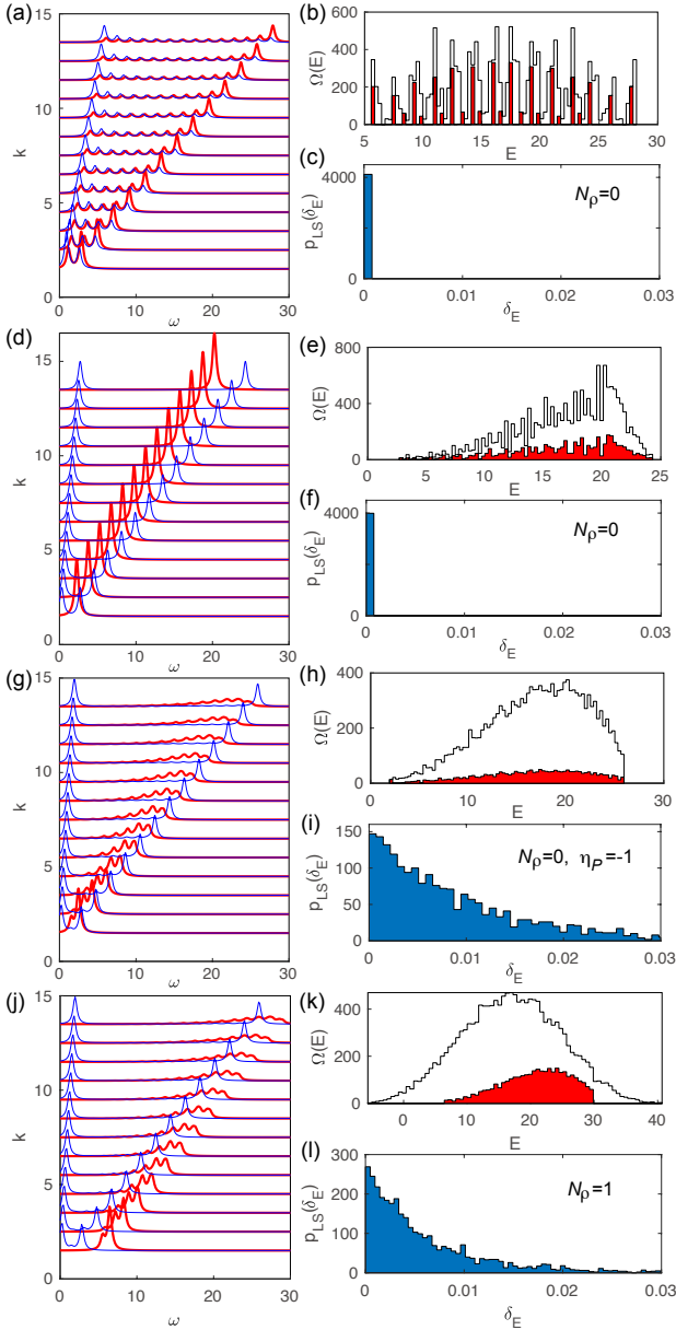
Figure 2: ED results up to total momentum K_{\text{tot}} = 13.5 for different parameters. We fix v_\rho = 1.5, v_n = 1 , and the other parameters are (a)-(c): J = 0, v_{n\rho} = 0.8, \mu_\rho = 0 ; (d)-(f): J = 0.8\pi, v_{n\rho} = 0, \mu_\rho = 0 ; (g)-(i): J = 0.8\pi, v_{n\rho} = 0.4, \mu_\rho = 0 , and (j)-(l): J = 0.8\pi, v_{n\rho} = 0.4, \mu_\rho = 4 . (a), (d), (g), (j) are spectral weight of fermions \rho (thick red lines) and n (thin blue lines). The upper unfilled (lower filled) lines in (b), (e), (h) show the total (the N_\rho = 0 subsector) DOS in the K_{\text{tot}} = 13.5 sector. The upper unfilled (lower filled) lines in (k) show the total (the N_\rho = 1 subsector) DOS in the K_{\text{tot}} = 13.5 sector. (c), (f) show the LSS of the ( K_{\text{tot}} = 13.5, N_\rho = 0 ) sector, in which cases the model is free. (i) shows the LSS of the ( K_{\text{tot}} = 13.5, N_\rho = 0, \eta_P = -1 ) sector. (l) shows the LSS of the ( K_{\text{tot}} = 13.5, N_\rho = 1 ) sector.
