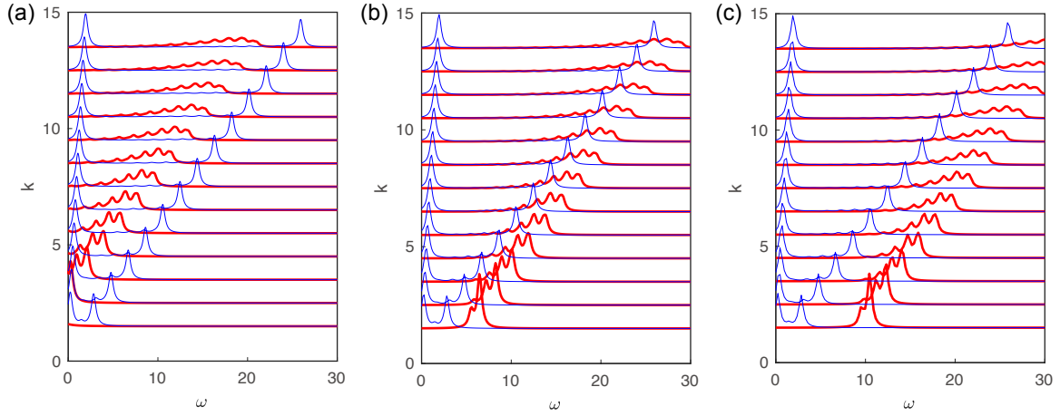
Figure 5: Spectral weights of n fermion (blue thin line) and \rho fermion (red thick line) up to total momentum K_{\text{tot}} = 13.5 . The parameters are J = 0.8\pi, v_{n\rho} = 0.4, v_\rho = 1.5, v_n = 1 for all cases but with different chemical potential: (a) \mu_\rho = -4 , (b) \mu_\rho = 4 , and (c) \mu_\rho = 8 .
