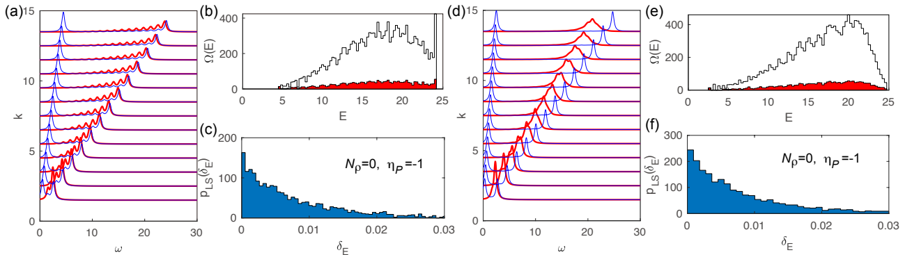
Figure 6: More ED results up to total momentum K_{\text{tot}} = 13.5 . We fix v_\rho = 1.5, v_n = 1, \mu_\rho = 0 , while the other parameters are given by (a)-(c): J = 0.6\pi, v_{n\rho} = 0.4 ; (d)-(f): J = 0.8\pi, v_{n\rho} = 0.2 . (a), (d) are the spectral weight of fermions \rho (thick red lines) and n (thin blue lines). The upper (lower) lines in (b), (e) show the total (the N_\rho = 0, \eta_P = -1 subsector) DOS in the K_{\text{tot}} = 13.5 sector. (c), (f) show the LSS of the ( K_{\text{tot}} = 13.5, N_\rho = 0, \eta_P = -1 ) sector.
