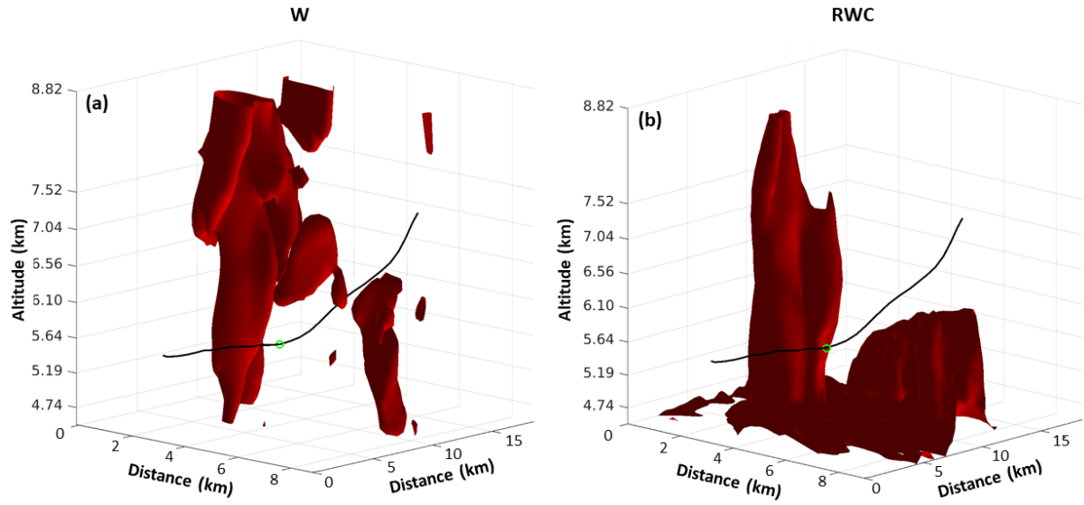
Figure 19: the trajectory of a specific air parcel (black line) and the location of the parcel at t = 0 min (green circle). The red surfaces in (a) show the area with w larger than 3 m/s, and in (b) with RWC larger than 0.05 \text{ g m}^{-3} , at the moment of t = 0 min.
