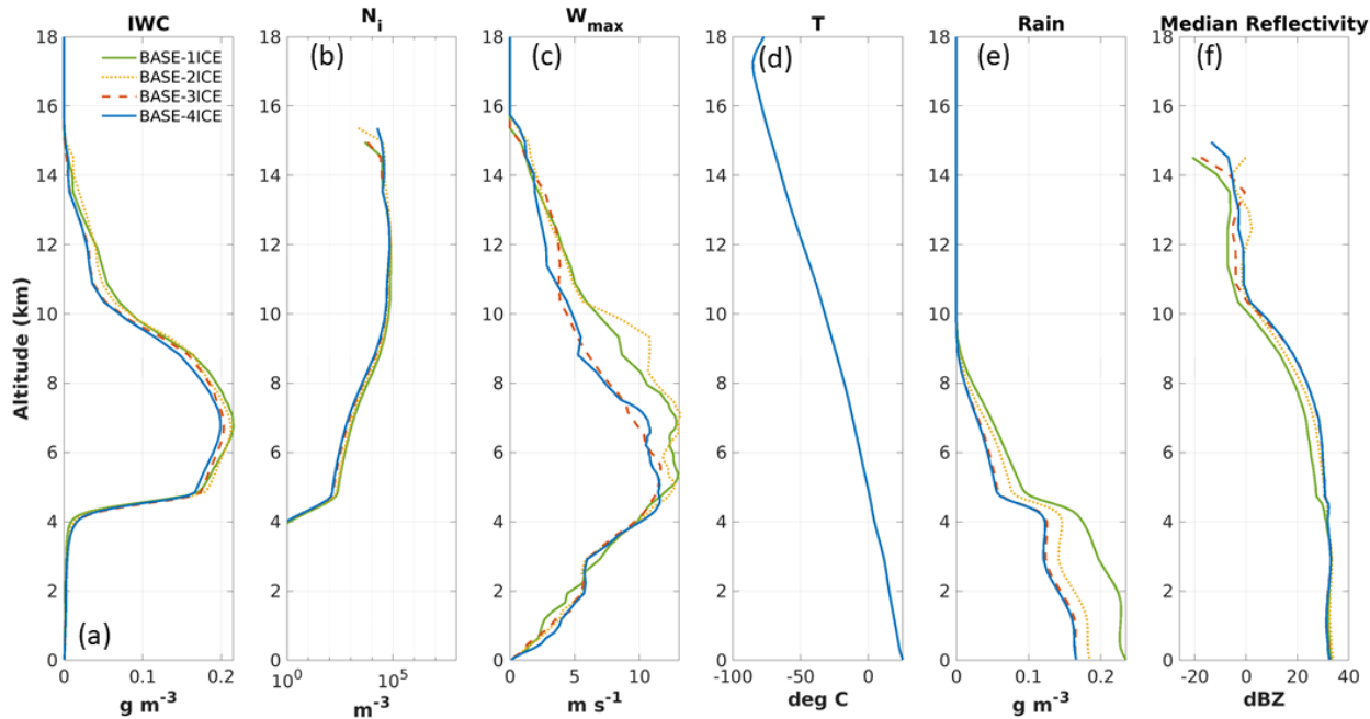
Figure 4: Profiles from the baseline simulations without SIP. (a): ice water content (IWC), (b): ice number concentration N_i , (c): maximum vertical wind speed W_{\text{max}} , (d) air temperature (the four simulations have only slightly different temperature that is not distinguishable in the figure) T, (e): rain water content RWC, (f): median radar reflectivity. The profiles are calculated based on data from 90 to 150 min of simulation. (a) and (b) are horizontally averaged over regions with \text{IWC} > 0.001 \text{ g m}^{-3} , (c) is the horizontal maximum across the domain, (d) is a horizontal average over the whole domain, (e) is an average over the area with both ice water path and rain water path larger than 1 \text{ g m}^{-2} , and (f) shows median values of reflectivity including points with either IWC or RWC larger than 0.01 \text{ g m}^{-3} within the mask used for (e).
