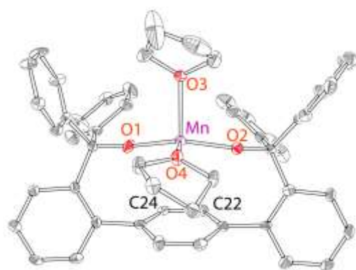
Figure 1. X-ray structure (50% probability) of Mn[O-terphenyl-O] Ph (THF) 2 ( 2 ). Alternative conformations of one of the top THF ligands and one of the lateral phenyls, H atoms, and disordered solvent were omitted for clarity. Selected bond distances (Å) and angles (°): Mn-O1 1.888(5), Mn-O2 1.922(4), Mn-O3 2.205(4), Mn-O4 2.178(4), O1-Mn-O2 150.3(2), and O3-Mn-O4 91.23(2).
