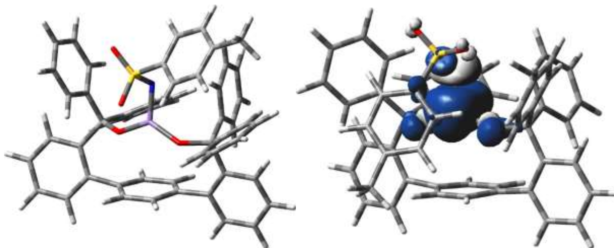
Figure 3. Optimized structure of the lowest energy quartet (left) and its spin density isosurface plotted using a cutoff value of 0.002 au (right). Blue and white surfaces correspond to excess alpha and beta spins, respectively.
