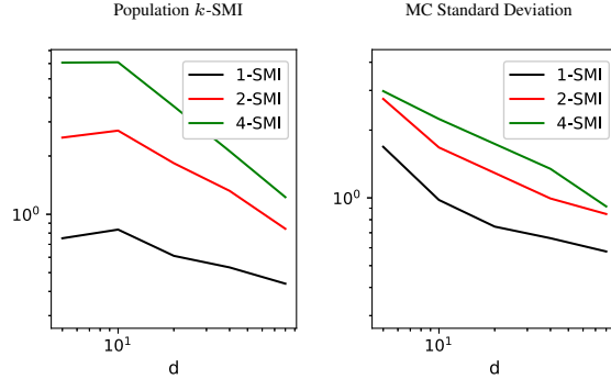
Figure 1: Decay with dimension the population k -SMI (left) and the associated MC standard deviation (right).
