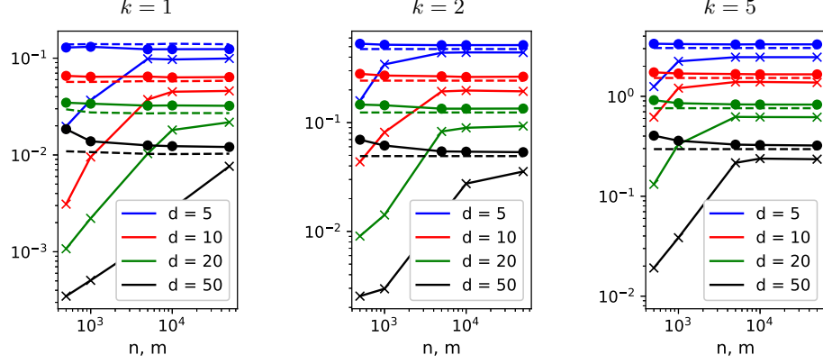
Figure 3: Neural estimation rates: Dashed line shows the ground truth, circle line is the value of the parallel neural estimator from Section 4.2, and the cross line is the SMI neural estimator from [17]. The parallel neural estimator converges at a faster rate for all considered k and d .
