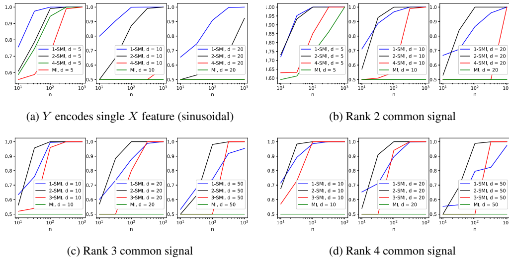
Figure 2: Independence testing with k -SMI: AUC ROC versus sample size n for different k and d .
