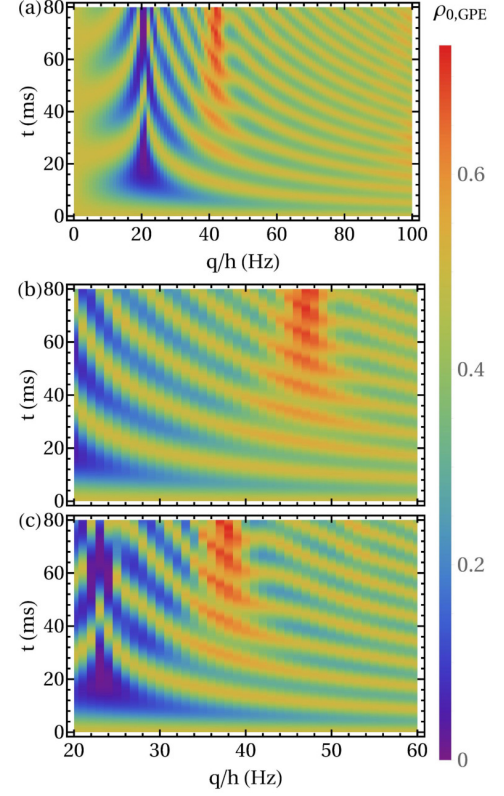
FIG. 3: Fractional population \rho_{0,\text{GPE}}(t) as functions of time t and Zeeman energy q for \omega_z = 2\pi \times 246 Hz, \omega_\rho = 2\pi \times 140 Hz, and (a) N = 2.3 \times 10^4 , (b) N = 1.7 \times 10^4 , and (c) N = 3.1 \times 10^4 ; the color coding is given by the color bar on the right. In (a), the oscillation period diverges at q/h \approx 20 Hz, in agreement with the mean-field SMA result of q/h \approx c_s/h = 20.9 Hz. Note that the range of q values considered in (a) is larger than in (b) and (c). This paper focuses on the regime where the spin dynamics deviate from regular oscillatory behaviors; the red color for q/h \approx 40 Hz signals drifting. It can be seen that the q -values for which the drifting occurs (“fuzzy” red region) move to smaller values with increasing N .
