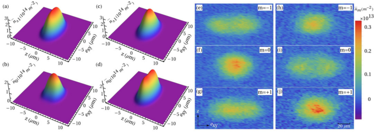
FIG. 9: Theoretical and experimental spatial integrated two-dimensional densities \bar{n}_m [defined through \bar{n}_m(e_{xy}, z, t) = \int n_m(\vec{r}, t) d\eta , where \eta = (x + y)/\sqrt{2} ] for q/h = 31 Hz. (a)-(d) Theoretical densities, obtained by solving the coupled Gross-Pitaevskii equations for N = 4 \times 10^4 , \omega_\rho = 2\pi \times 140 Hz, and \omega_z = 2\pi \times 246 Hz; (a) m = \pm 1 and t = t_{\text{hold}} = 50 ms, (b) m = 0 and t = t_{\text{hold}} = 50 ms, (c) m = \pm 1 and t = t_{\text{hold}} = 58 ms, and (d) m = 0 and t = t_{\text{hold}} = 58 ms. The normalization is \sum_m \int n_m(\vec{r}, t) d\vec{r} = N . The time-of-flight sequence is not included in the simulations. (e)-(j) Experimental two-dimensional images for 10.5 ms time-of-flight expansion; (e) m = -1 and t = t_{\text{hold}} = 50 ms, (f) m = 0 and t = t_{\text{hold}} = 50 ms, (g) m = +1 and t = t_{\text{hold}} = 50 ms, (h) m = -1 and t = t_{\text{hold}} = 58 ms, (i) m = 0 and t = t_{\text{hold}} = 58 ms, (j) m = +1 and t = t_{\text{hold}} = 58 ms. The particle numbers N are 2.6 \times 10^4 and 2.2 \times 10^4 for (e)-(g) and (h)-(j), respectively. To aid with the visualization, the three images were centered individually. The side bar on the right defines the color code for the experimental images shown in (e)-(j).
