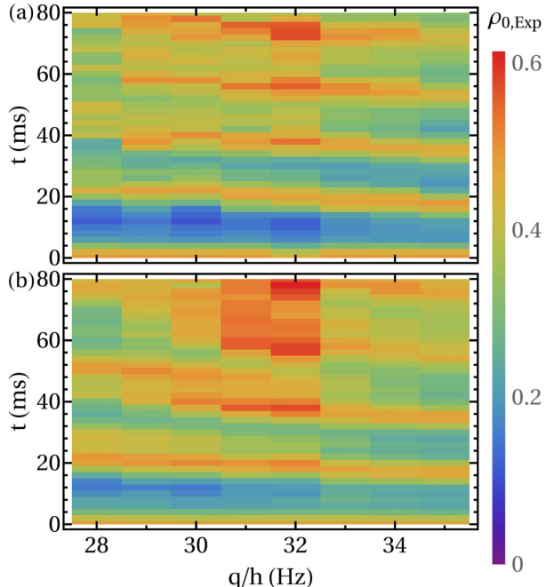
FIG. 6: Fractional population \rho_{0,\text{Exp}} as functions of the hold time t = t_{\text{hold}} and the Zeeman energy q/h determined in two different experimental campaigns. The trap frequencies are (a) (\omega_x, \omega_y, \omega_z) = 2\pi \times (147, 132, 246) Hz and (b) (\omega_x, \omega_y, \omega_z) = 2\pi \times (140, 122, 255) Hz. The red regions are interpreted as signatures of the drifting, in qualitative agreement with what is predicted by mean-field Gross-Pitaevskii simulations (see Fig. 3).
