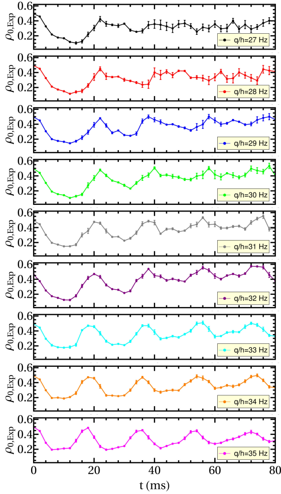
FIG. 7: Fractional population \rho_{0,\text{Exp}}(t) (symbols) as a function of t for various q/h , as indicated by the label in each panel. The \rho_{0,\text{Exp}} data are identical to those shown in Fig. 6(a). Error bars indicate the standard deviation calculated from ten independent experimental runs.
