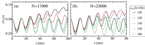
FIG. 5: Fractional population \rho_{0,\text{GPE}}(t) as a function of time t for q/h = 40 Hz, \omega_z = 2\pi \times 246 Hz, and (a) N = 1.7 \times 10^4 and (b) N = 2.3 \times 10^4 . The different lines show results for different \omega_\rho , ranging from 2\pi \times 120 to 2\pi \times 160 Hz (see the legend on the right of the figure).
