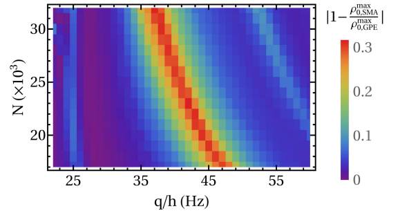
FIG. 4: Absolute value of the normalized difference [\rho_{0,\text{GPE}}^{\max} - \rho_{0,\text{SMA}}^{\max}]/\rho_{0,\text{GPE}}^{\max} , obtained by considering 0 < t \leq 80 ms, as functions of N and q/h for \omega_z = 2\pi \times 246 Hz and \omega_\rho = 2\pi \times 140 Hz.
