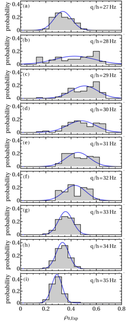
FIG. 8: Distribution of fractional population \rho_{0,\text{Exp}} at t = t_{\text{hold}} = 60 ms for (\omega_x, \omega_y, \omega_z) = 2\pi \times (147, 132, 246) Hz for (a) q/h = 27 Hz to (i) q/h = 35 Hz. The blue lines show Gaussian distributions, using the mean value and standard deviation of the experimentally measured \rho_{0,\text{Exp}} .
