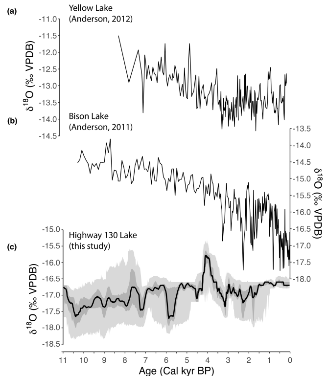
Figure 6. \delta^{18}\text{O}_{\text{carb}} records from (a) Yellow Lake (Anderson, 2012), (b) Bison Lake (Anderson, 2011), and (c) Highway 130 Lake. In panel (c) the black line represents the median estimate of the ensemble regression, and the dark and light gray bands show the 50 % and 95 % highest-probability density regions, respectively.
