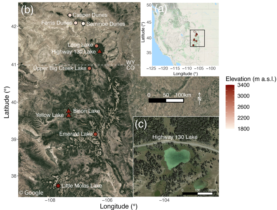
Figure 1. Locations of the study site and related climate records. (a) Highway 130 Lake (triangle; this study) and related carbonate (triangles), dune-field chronology, pollen, and lake-level records (circles) lie within the southern Rocky Mountains, a critical headwater area in the western United States that contributes snowmelt to the Colorado and North Platte rivers. (b) Study site locations in the Colorado Front Range and Medicine Bow Mountains, southeastern Wyoming. (c) Highway 130 Lake lies within the Snowy Range, a subsection of the Medicine Bow Mountains. Google images (© Google Maps 2021) were acquired using the ggmap package in R (Kahle and Wickham, 2013).
