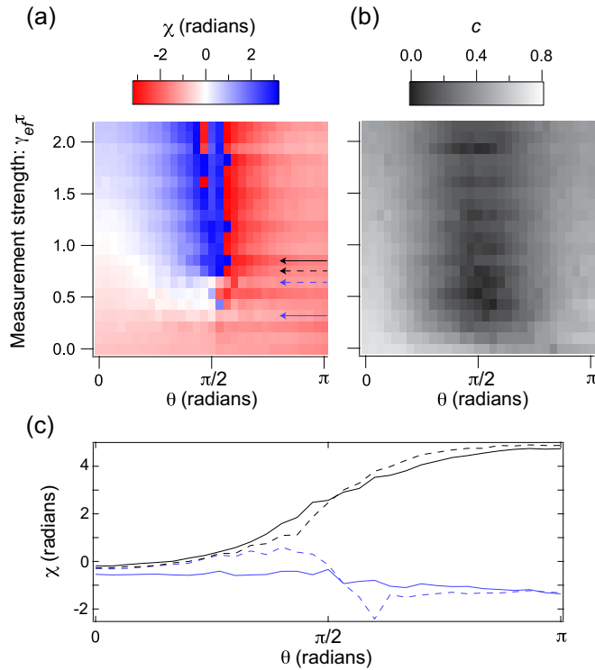
FIG. 4. (a) The geometric phase under varying measurement strength ( \gamma_{eff}\tau ) gained with sequential measurements along different latitudes of the Bloch sphere for polar angle 0 \rightarrow \pi . The black (blue) arrows mark measurement strengths above (below) the transition. (b) The corresponding contrast of the interference vanishes at the transition. (c) The geometric phase along fixed measurement strengths before the transition (blue lines), where the set of trajectories does not wrap the Bloch sphere, and after the transition (black lines) where the set of trajectories wraps the Bloch sphere.
