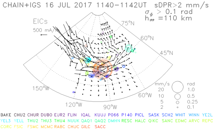
Fig. 32 Horizontal equivalent ionospheric currents observed over North America on 16 July 2017. IPPs where \sigma_\phi > 0.1 rad or sDPR > 2 mm/s are shown as circles colour coded by stations and sized proportionally to \sigma_\phi and sDPR values
