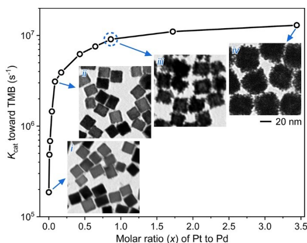
Figure 4. Effect of Pt content on the peroxidase-like catalytic efficiency of Pd@Pt NDs. A plot comparing the K_{cat} values toward TMB of Pd@Pt NDs with different molar ratios ( x ) of Pt to Pd (i.e., Pd@Pt x NDs, x=0 –3.44). Insets show the TEM images of four representative Pd@Pt x NDs with x=0 (i), 0.0860 (ii), 0.860 (iii), and 3.44 (iv).
