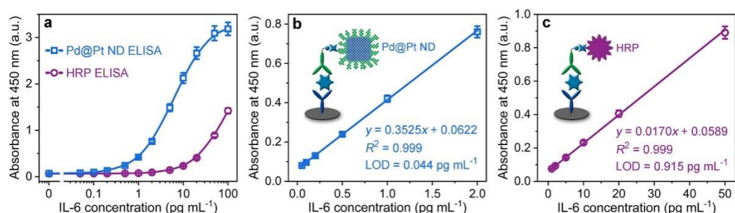
Figure 6. Detection of IL-6 standards using the colorimetric Pd@Pt ND ELISA (blue curve) and conventional HRP ELISA (violet curve). (a) Calibration curves of Pd@Pt ND ELISA and HRP ELISA that were generated by plotting the absorbance at 450 nm of the final detection solution against IL-6 concentration. (b,c) Linear range regions of the calibration curves for Pd@Pt ND ELISA (b) and HRP ELISA (c).
