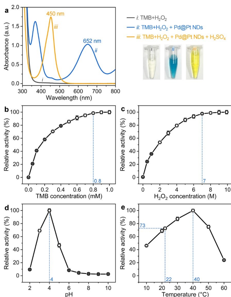
Figure 2. Verification and optimization of the peroxidase-like catalytic activity of Pd@Pt NDs. (a) UV-vis spectra of TMB+H 2 O 2 substrate solution (i), (TMB+H 2 O 2 )+Pd@Pt NDs solution (ii), and (TMB+H 2 O 2 )+Pd@Pt NDs+H 2 SO 4 solution (iii). The bottom-right panel shows the corresponding photographs taken from the three solutions. (b–e) Effect of TMB concentration (b), H 2 O 2 concentration (c), pH (d), and temperature (e) on the peroxidase-like catalytic activity of Pd@Pt NDs. The maximum point in each curve is set as 100%.
