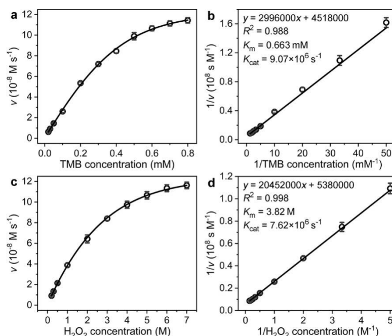
Figure 3. Steady-state kinetic analysis of the peroxidase-like catalytic activity of Pd@Pt NDs. (a, b) Kinetic analysis toward TMB: (a) plot of v versus TMB concentration, in which 7.0 M \text{H}_2\text{O}_2 was used; (b) double-reciprocal plot converted from (a). (c, d) Kinetic analysis toward \text{H}_2\text{O}_2 : (c) plot of v versus \text{H}_2\text{O}_2 concentration, in which 0.8 mM TMB was used; (d) double-reciprocal plot converted from (c).
