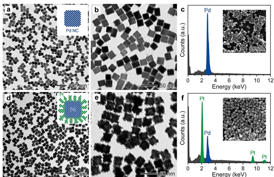
Figure 1. Characterization of 18 nm Pd NCs and Pd@Pt NDs. (a,b) Low- (a) and high- (b) magnification TEM images of 18 nm Pd NCs. (c) EDX spectrum of 18 nm Pd NCs deposited on a silicon substrate. (d,e) Low- (d) and high- (e) magnification TEM images of Pd@Pt NDs. (f) EDX spectrum of Pd@Pt NDs deposited on a silicon substrate. Insets in (c, f) show the corresponding scanning electron microscope (SEM) images of the region where the EDX spectra were acquired.
