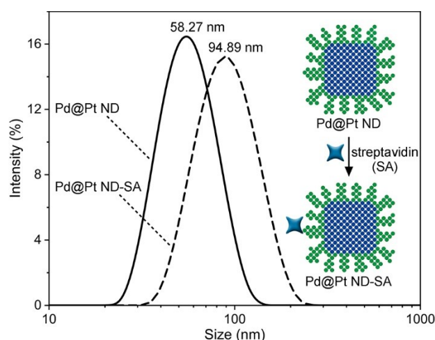
Figure 5. Characterization of Pd@Pt ND-SA conjugates. DLS size distributions of Pd@Pt NDs (solid curve) and Pd@Pt ND-SA conjugates (dashed curve) dispersed in DI water.
