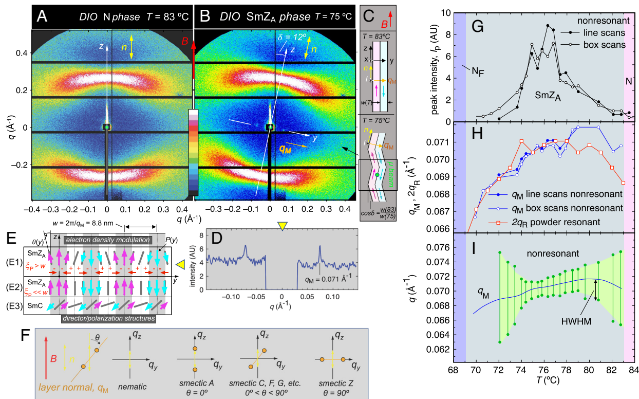
Fig. 2. SAXS scattering from the N and SmZ A phases of DIO. These diffractograms are from a sample in a 1 mm-diameter capillaries in which the director, n , is aligned along the magnetic field B (red), studied on the SMI microbeam line at NSLS II. (A and B) Non-resonant diffractograms obtained on cooling show a diffuse scattering arc at q_z = 0.25 \text{ \AA}^{-1} from head-to-tail stacking of the molecules in the N and SmZ A phases. In the SmZ A phase, equatorial Bragg spots appear, indicating the presence of an electron density wave of w_M = 8.8\text{-nm} periodicity, with wavevector q_M normal to n . These peaks disappear upon transitioning to the N F phase (G, SI Appendix, Figs. S4 and S5). (C) The scattering pattern rotates from (A) to (B) because of layer reorientations caused by a small reduction in layer thickness upon cooling in the SmZ A phase (see text). (D) Line scan through the non-resonant scattering peaks. The central part of the beam is blocked by the beam stop. (E) Since the sample is a powder in orientation about the B field, the observed scattering pattern could be indicative of either lamellar or hexagonal columnar positional ordering. Since non-resonant scattering is sensitive only to electron density, the layers (of thickness w_M ) of opposite polarization scatter identically. Layer boundaries (white stripes) have different electron density than the layer centers (gray stripes), making w_M the period observed in nonresonant scattering. However, as shown in (H) and SI Appendix, Fig. S5, carbon-edge resonant scattering exhibits the half-order peak at q_R = q_M/2 , showing conclusively that the SmZ A is lamellar and bilayer with period 2w_M . The DTOM experiments show that it is lamellar and antiferroelectric, with layers of alternating polarization P(y) , sketched in (E1) for low polarization ( \xi_p > w ), and in (E2) for high polarization ( \xi_p < w ), the case relevant to the SmZ A (see text). The tilt modulation \theta(y) is suppressed at large P by the self-electric field due to the polarization charge, \rho = -\nabla \cdot P , indicated in red. Other smectic structures (e.g., the SmC, sketched in E3) have spontaneous antiferroelectric polarization in the tilt plane as well as splay modulation SI Appendix, Section 8), but in different geometries. (F) X-ray scattering peaks from various smectics with the director aligned by the magnetic field B . (G–I) Dependence on T of the Bragg peak parameters from data as in SI Appendix, Figs. S4 and S5 [non-resonant peak intensity ( I_p ), non-resonant peak position ( q_M = 2\pi/w_M ), resonant peak position ( q_R = 2\pi/2w_M ), and non-resonant half-width at half-maximum (HWHM M )]. (H) Layers of opposite P have different carbon K-edge resonant scattering cross-sections, and therefore Bragg scatter at the full antiferroelectric period 2w_M . (I) The HWHM M values of the mid-range peaks ( T \sim 75^\circ\text{C} ) are SAXS-resolution limited.
