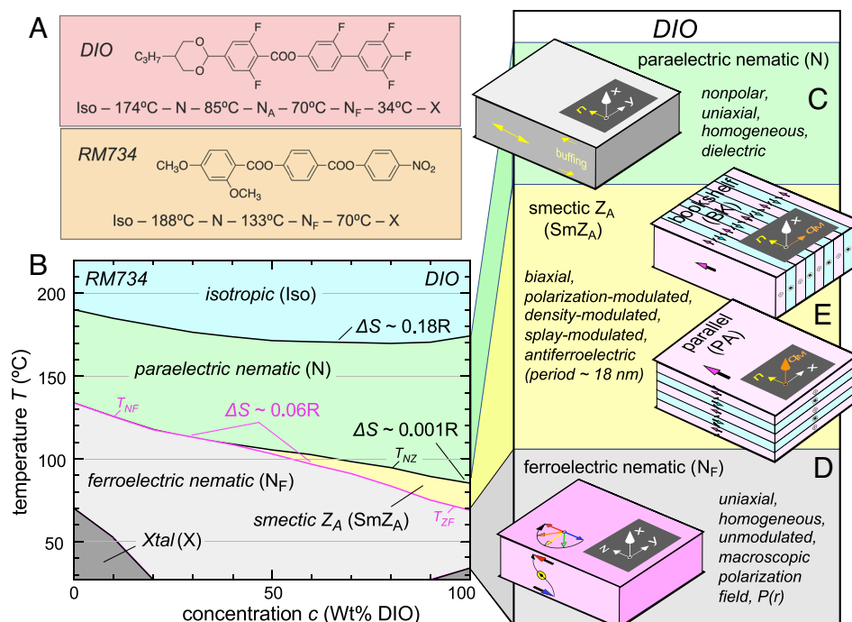
Fig. 1. (A) Representative members DIO [2,3',4',5'-tetrafluoro-[1,1'-biphenyl]-4-yl 2,6-difluoro-4-(5-propyl-1,3-dioxane-2-yl) benzoate] and RM734 [4-[(4-nitrophenoxy) carbonyl]phenyl-2,4-dimethoxybenzoate] of nitro- and fluoro-based molecular families of molecules that exhibit the ferroelectric nematic phase. This behavior is attributable in part to their rod-like molecular shape, large longitudinal dipole moment, and a common tendency for head-to-tail molecular association. (B) Phase diagram of DIO and RM734 and their binary mixtures exhibiting: (C) Paraelectric nematic (N) phase, in which the molecular long axes are aligned in a common direction but with no net polarity, making a nonpolar phase with a large dielectric response. (D) Ferroelectric nematic (N F ) phase, in which the polar orientation of dipoles is unidirectional and long-ranged, with a large polar order parameter ( \sim 0.9 ). The N F phase is uniaxial and spatially homogeneous, with a macroscopic polarization/director field P(r) , shown here for antiparallel polar orienting surface alignment layers on the plates (9). The phase diagram shows that the transition temperature into the N F depends nearly linearly on concentration c , indicating that these molecules exhibit near ideal mixing behavior of the transition into the ferroelectric nematic (N F ) phase. This transition is weakly first-order, with entropy \Delta S \approx 0.06R . (E) Intermediate phase observed in neat DIO and in DIO-rich mixtures. Originally called the M2 (6), we find this phase to be electron density-modulated into \sim 9 -nm thick, polar layers, in which the director and polarization are parallel to the layer plane and alternate in direction from layer to layer, as sketched. We have termed this lamellar, antiferroelectric phase the smectic Z A (SmZ A ). The SmZ A can be prepared with the layers either normal to the plates (bookshelf geometry) or parallel to the plates, or with the chevron texture shown in Figs. 2 and SI Appendix Figs. 6–8.
