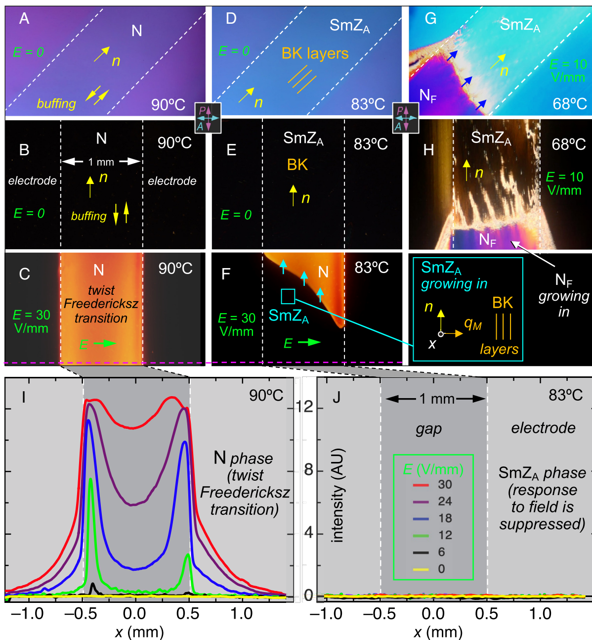
Fig. 3. Textures of DIO in a d = 3.5\text{-}\mu\text{m} cell with in-plane electrodes spaced by 1 mm and antiparallel buffing parallel to the electrode edges, cooled at -1\text{ }^{\circ}\text{C}/\text{min} and viewed in DTOM with polarizer and analyzer as indicated. (A–C) Planar-aligned nematic monodomain with n parallel to the plates and to the electrode edges, showing (A) a birefringence color corresponding to d = 3.5 and \Delta n = 0.18 , (B) excellent extinction with n parallel to the polarizer, and (C) the transmission due to twist of n during a field-induced twist Fredericksz transition. (D and E) Bookshelf-aligned (BK) smectic Z_A monodomain formed on cooling. The smectic layers are parallel to n and normal to the cell plates. The birefringence is slightly larger than in the nematic phase and excellent extinction is again obtained with n parallel to the polarizer. (F) Optical response of coexisting nematic and \text{Sm}Z_A phases to an applied 200-Hz square wave field of peak amplitude, E . The nematic region undergoes a twist Fredericksz transition but in the smectic Z_A phase, rotation of the director is suppressed by the layering. (G and H) N_F phase growing into the \text{Sm}Z_A upon further cooling. The antiparallel buffing stabilizes a \pi -twist state in the polarization/director field of the N_F , which does not extinguish between crossed polarizer and analyzer at any cell orientation. (I and J) Optical intensity scans along the magenta dashed lines across the bottom of the images in (C and F), probing the electric field-induced in-plane twist Fredericksz reorientation in the N_F phase and showing that there is no observable electro-optic effect in the \text{Sm}Z_A phase. In this geometry, where the layers have bookshelf (BK) alignment, an in-plane field would tend to rotate the director out of the smectic layer planes, a deformation that is locally resisted by the \text{Sm}Z_A structure.
