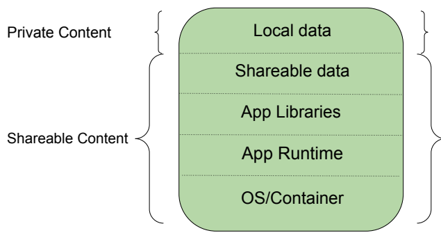
Fig. 3. Function Execution Stack. This graph is especially for concurrent functions of an application that can share data according to [11]
