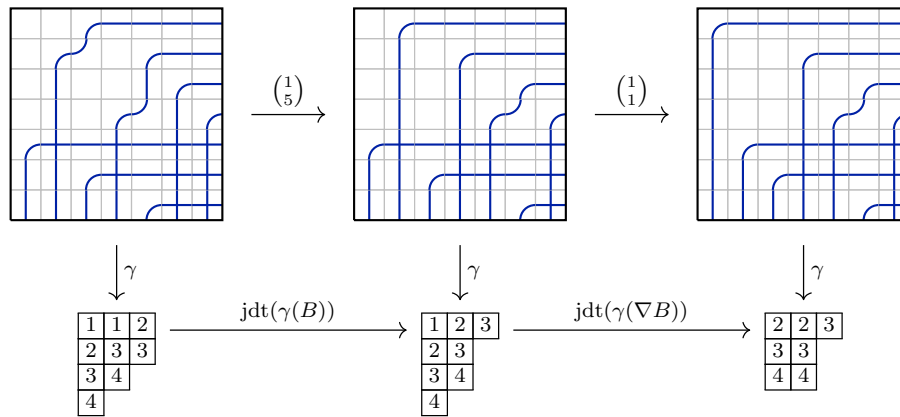
Figure 3: An illustration of Proposition 8.
