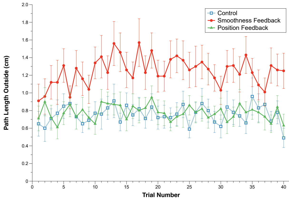
Fig. 5. Average path length outside the figure as a function of condition and trial. Error bars show standard error of the mean. The average standard error of the mean across all conditions was 0.15.
