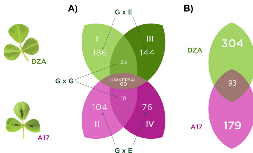
FIG 1 Association mapping of partner quality reveals strong signatures of environmental-dependence. Venn diagram showing number of rhizobium ( S. meliloti ) genes significantly associated with plant ( M. truncatula ) aboveground biomass (one metric of symbiotic partner quality) in (A) each of four separate mapping experiments with either host line DZA (I and III in green) or host line A17 (II and IV in pink). Green and pink unions represent genes contributing to plant biomass in both experiments with either DZA or A17, respectively, while the mauve oval in the center represents universal genes found to contribute to plant aboveground biomass in at least three of the four experiments. (B) Genes significantly associated with cross-experiment plasticity in plant aboveground biomass for host genotype DZA in green (experiments I versus III), A17 in pink (experiments II versus IV), or independently associated with plasticity in both hosts (central mauve triangle).
