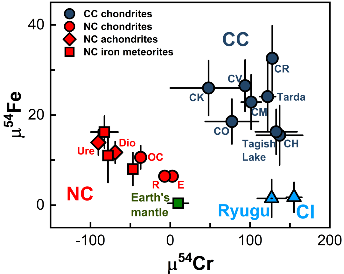
Fig. S3. Isotopic anomalies of Fe and Cr in Ryugu and other Solar System materials. The average \mu^{54}\text{Fe} and \mu^{54}\text{Cr} data of Ryugu samples are from this study and Yokoyama et al. (6). The average compositions of non-carbonaceous (NC) and carbonaceous (CC) meteorite groups and Earth's mantle (BSE) are given in the data compilation Table S1 and are calculated using data from this study and the data compilation of Burkhardt et al. (64). Uncertainties for individual groups are the 95% confidence interval of the mean. E-enstatite; R-rumuruti; OC-ordinary chondrites; Ure=ureilites; Dio=diogenites. Error bars are smaller than symbols if not visible.
