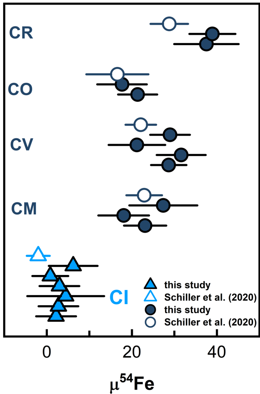
Fig. S1. Comparison of \mu^{54}\text{Fe} values of carbonaceous chondrites determined in this study with literature data of Schiller et al. (22). The data from this study agree with previous studies. Uncertainties of individual samples are 95% confidence intervals calculated from replicate analysis (N=14-30).
