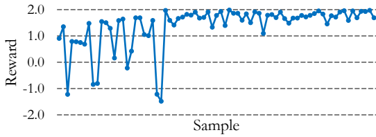
Fig. 18: Rewards over time using CEM.
