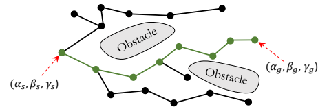
Fig. 10: Arm manipulator planning by the RRT algorithm.
