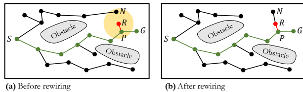
Fig. 11: A rewiring example with RRT* .
