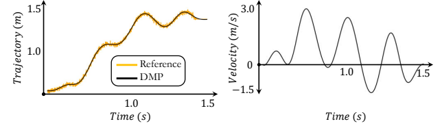
Fig. 15: Dynamic movement primitives.
