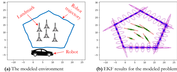
Fig. 3: SLAM using Extended Kalman Filter .
