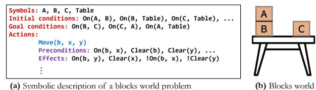
Fig. 13: Blocks world problem.
