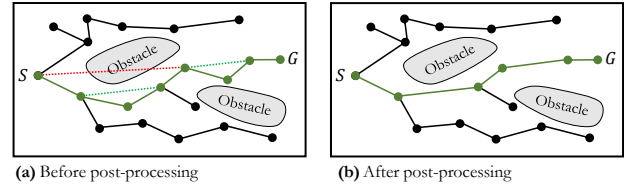
Fig. 12: Post-processing the path found by RRT .
