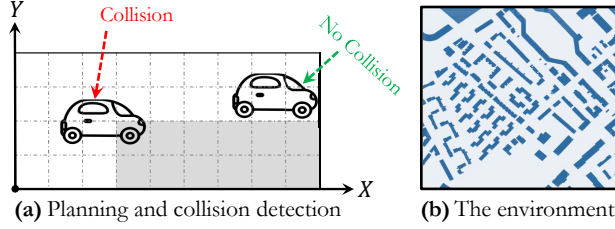
Fig. 5: 2D path planning.
