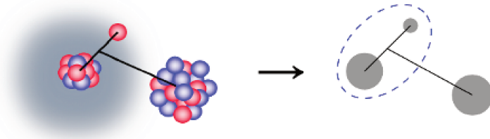
Fig. 3 Reduction of the many-body problem into a few-body one.
