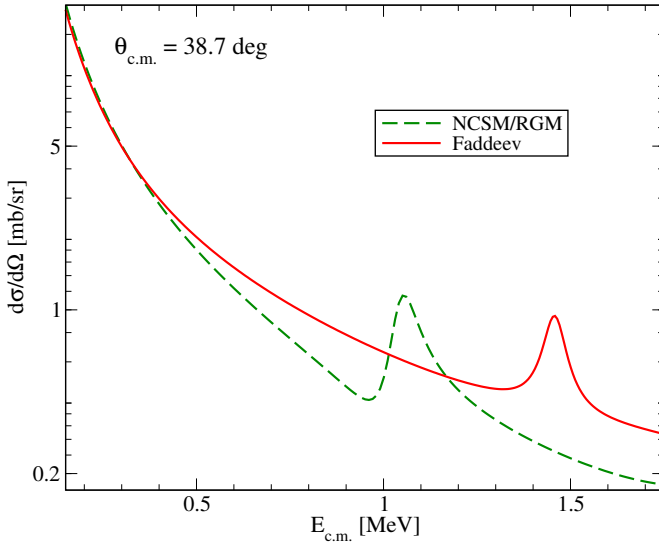
Fig. 7 The differential cross section for elastic d + \alpha scattering as a function of the center-of-mass energy E_{\text{c.m.}} at the scattering angle \theta_{\text{c.m.}} = 38.7 deg. The dashed lines shows phase shifts computed using the NCSM/RGM while the Faddeev results are depicted by solid lines. The model space for the Faddeev calculation is restricted to a total two-body angular momentum of \mathcal{I}_{n+p} \leq 3 and \mathcal{I}_{N+\alpha} \leq 9/2 for the n+p and N-\alpha subsystems. The NCSM/RGM model space is truncated at N_{\text{max}} = 12/13 for the positive/negative parity partial waves and \hbar\Omega = 14 MeV.
