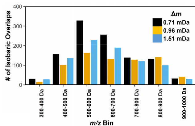
Figure 4. Number of isobaric overlaps in SRFA peak-picked at 3 \sigma identified in Figure 3 and binned by every m/z 100, up to m/z 1000. Bars are colored by theoretical isobaric overlap that each count was associated with. For the 4 \sigma , 5 \sigma , and 6 \sigma bar plots of the selected isobaric overlaps, see Figure S3.
