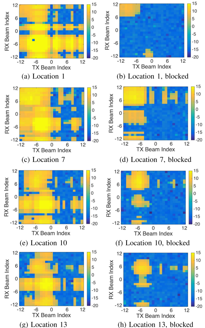
Fig. 11. SNR heatmaps for all beam pair combinations for user location indices 1, 7, 10 and 13 in the lobby under LOS connectivity (left column) and blockage (right column).
