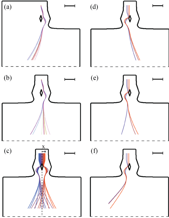
FIG. 3. Simulated droplet trajectories in the hydrodynamic pilot-wave system. In (a)–(c), the vibrational acceleration \gamma = 0.905\gamma_F . (a) When only one reflector is present, the droplet follows the expected trajectory, regardless of the initial conditions. (b) In the presence of a second reflector, depending on the initial conditions and the system memory, the droplet may follow a “surreal” trajectory, and so never cross the centerline. (c) An ensemble of initially vertical trajectories with different values of the impact parameter x . (d)–(f) The dependence on memory of a trio of originally vertical trajectories. As the memory parameter is increased from (d) 0.88\Gamma_F to (e) 0.9\Gamma_F to (f) 0.92\Gamma_F , all trajectories transform from expected to surreal. Scale bar: 5\lambda_F .
