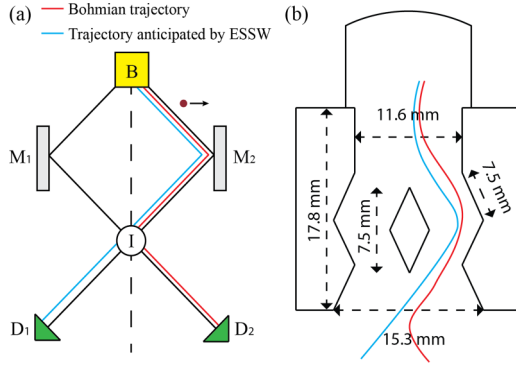
FIG. 1. (a) A variant of the interferometer setup considered by ESSW [6]. An incoming wave packet is split by a beam splitter B and reflected by the mirrors M_1 and M_2 . The wave packets interfere in the region I and then move towards the detectors D_1 and D_2 . The blue path represents the particle trajectory anticipated by ESSW, while the red path is that predicted by Bohmian mechanics. The red dot represents the one-bit, which-way detector. (b) Our experimental arrangement. A walking droplet is released from a launching area towards a beam splitter that directs the droplet towards one of two submerged barriers with equal probability. The blue and red paths are the possible analogs of those in the ESSW setup.
