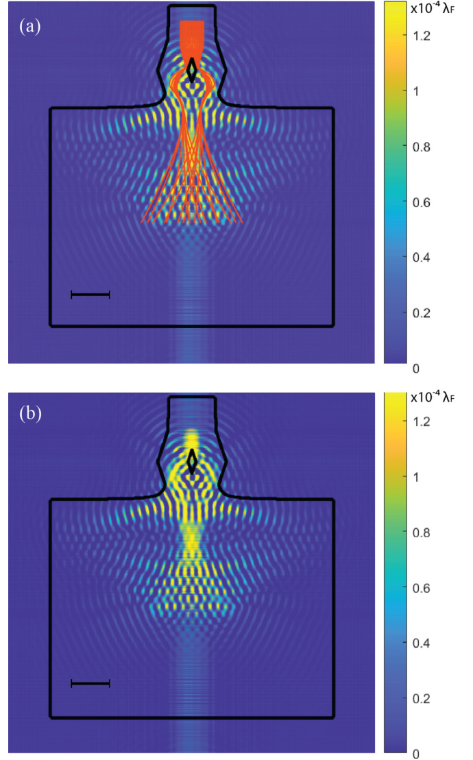
FIG. 4. The mean wave field generated by averaging simulated droplet trajectories with a Gaussian distribution of initial impact parameters, with a standard deviation of 1.4\lambda_F , (a) with and (b) without the associated droplet trajectories overlaid. The wave amplitude is presented in units of the system’s Faraday wavelength. Scale bar: 5\lambda_F .
