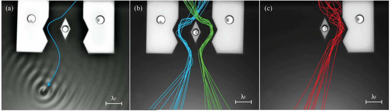
FIG. 2. Droplet trajectories in the hydrodynamic pilot-wave system. (a) A single-particle trajectory, along with the pilot-wave field at the instant that the drop is at the position shown. (b) In a symmetric setup, the droplet enters the right or left channel with equal probability, after which it is deflected away from the system centerline, resulting in a “surreal” trajectory. Twenty such trajectories are shown. (c) When one of the barriers is removed, the symmetry of the system is broken. The walking droplet is then reflected away from the remaining barrier, resulting in the trajectory that one might expect.
