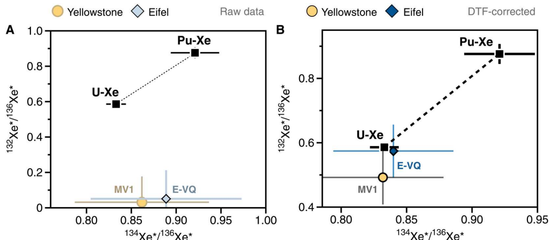
Fig. 7. ^{132}\text{Xe}^*/^{136}\text{Xe}^* versus ^{134}\text{Xe}^*/^{136}\text{Xe}^* systematics of Yellowstone and Eifel samples with the highest mantle contributions reported in this study (i.e., MV1 and E-VQ, respectively), before and after DTF correction. (A and B) The pure uranium (U-Xe) and plutonium (Pu-Xe) fissionogenic end-members (17) are shown as black squares. Once corrected for DTF, MV1 and E-VQ samples both appear most consistent with fissionogenic Xe isotopes deriving from uranium.
