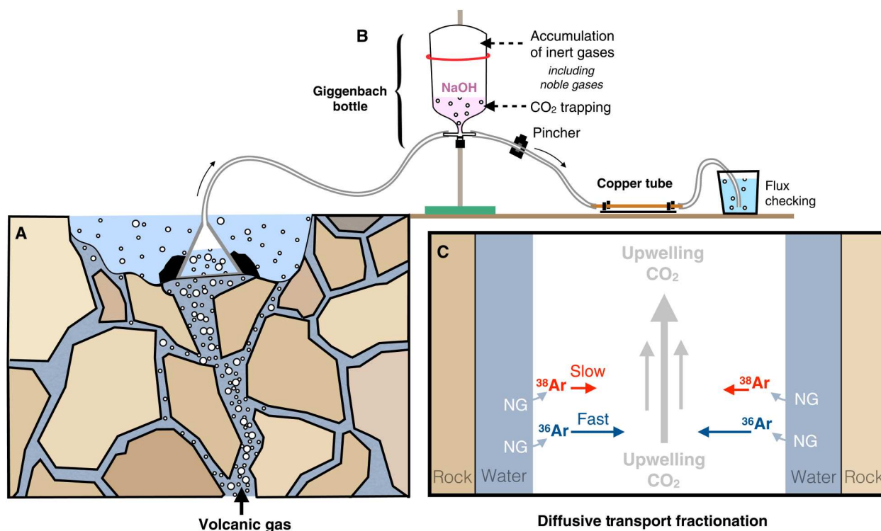
Fig. 3. Schematic representation of typical volcanic gas collection and illustration of DTF. (A to C) Cross-section of the subsurface, where volcanic gas (mainly \text{CO}_2 ) ascends through shallow groundwater until it reaches the surface. Part of the gas is captured by an upside-down funnel submerged in surficial water. The captured gas then flows through the tubing system and copper tube, until it reaches the preevacuated Giggenbach bottle containing a 5 N NaOH solution (17, 51). Because of the pressure gradient across the NaOH solution, a fraction of the volcanic gas is sucked into the Giggenbach bottle, where \text{CO}_2 dissolves in solution and inert gases accumulate in the headspace. \text{CO}_2 bubble stripping of groundwater-derived noble gases is a ubiquitous process that accounts for the occurrence of air-derived components with AEW elemental abundances in volcanic gas systems (Fig. 2) (45). Groundwater-derived noble gases then experience diffusive transport against \text{CO}_2 [also referred to as “binary” or “mutual” diffusion; (20, 26)]. The difference between the diffusion coefficients of heavy (slow) and light (fast) isotopes (here, only ^{36}\text{Ar} and ^{38}\text{Ar} are shown for illustrative purpose) produces a depletion of the heavy isotopes (in this case, ^{38}\text{Ar} ), whose magnitude depends on the atomic mass of the gas in medium (20).
