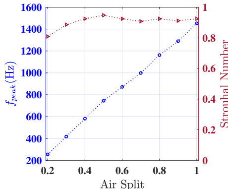
FIGURE 6. Peak frequency and Strouhal number as a function of air split for non-reacting conditions.
