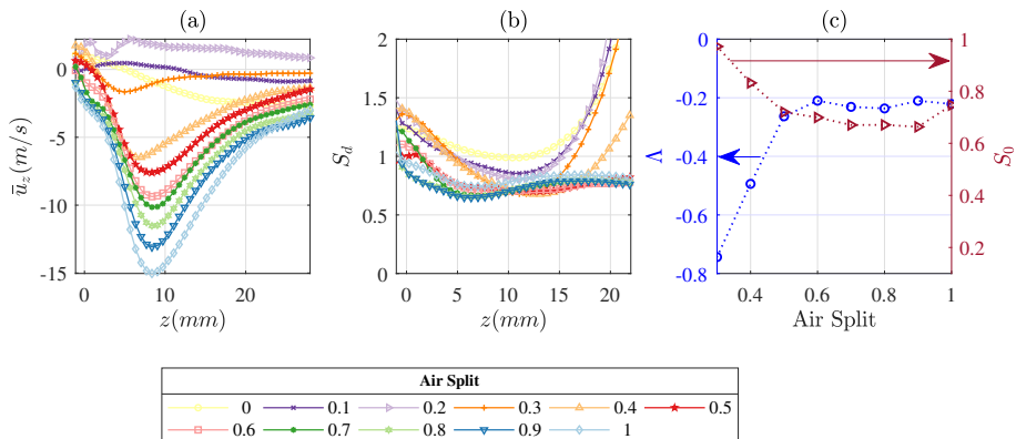
FIGURE 4. (a) Centerline time-averaged axial velocity, (b) swirl number, and (c) backflow ratio and swirl number at the downstream location of minimum mean centerline axial velocity for all air split conditions.
