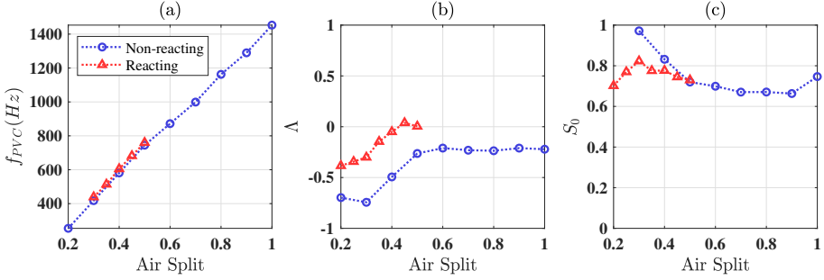
FIGURE 18. (a) Variation of PVC frequency with air split, (b) variation of backflow ratio with air split, and (c) variation in swirl number at the minimum centerline velocity location for both reacting and non-reacting conditions.
