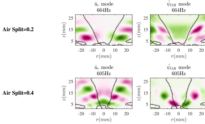
FIGURE 16. Spatial mode shapes for the radial velocity field and the OH-PLIF signal field obtained from composite spectral POD at the peak frequencies of leading modes for two air split conditions.
