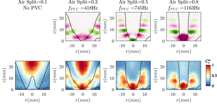
FIGURE 7. Spectral POD mode shapes corresponding to the PVC frequency (top row) with the critical region identified by the weighted closeness centrality measure (bottom row) from the complex network analysis computed for the transverse velocity component at various air splits.
