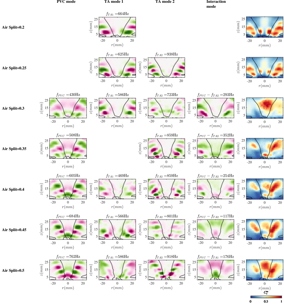
FIGURE 13. Spectral POD mode shapes at PVC, thermoacoustic, and interaction frequencies, and weighted closeness centrality measures computed for the radial velocity component at all air split conditions.
