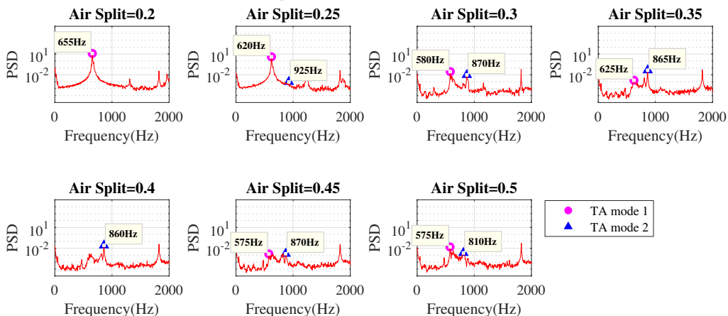
FIGURE 10. Acoustic pressure spectra at each air split condition.
