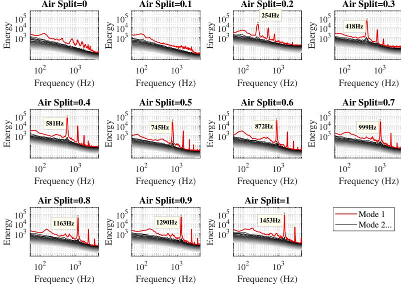
FIGURE 5. Modal energy spectra from SPOD for non-reacting conditions varying air splits.
