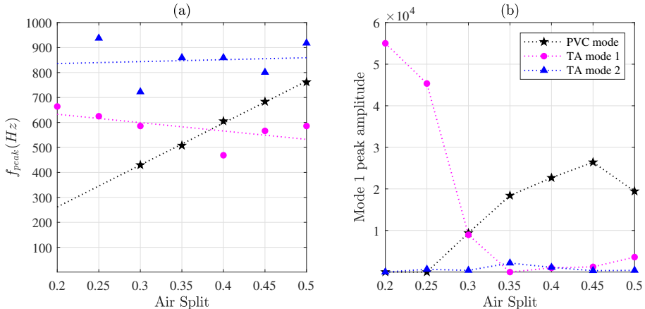
FIGURE 12. Frequency (a) and amplitude (b) characterization of the three oscillation modes seen at each air-split condition from SPOD.
