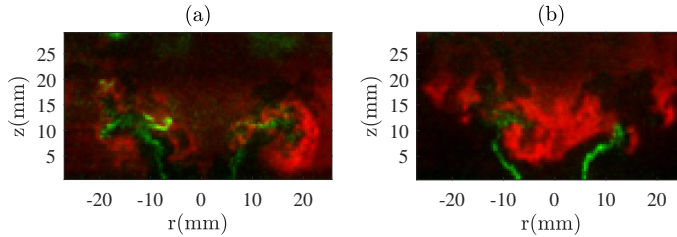
FIGURE 14. Instantaneous images of superimposed OH-PLIF (red) and acetone-PLIF (green) profiles at air splits 0.25 (a) and 0.5 (b). Videos of these conditions are provided in the supplemental material.
