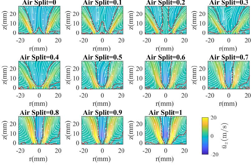
FIGURE 3. Time-averaged streamwise velocity for all non-reacting conditions with streamlines, depicted as white curves and the limits of the recirculation zone ( \bar{u}_z = 0 ) depicted with dotted red contours.
