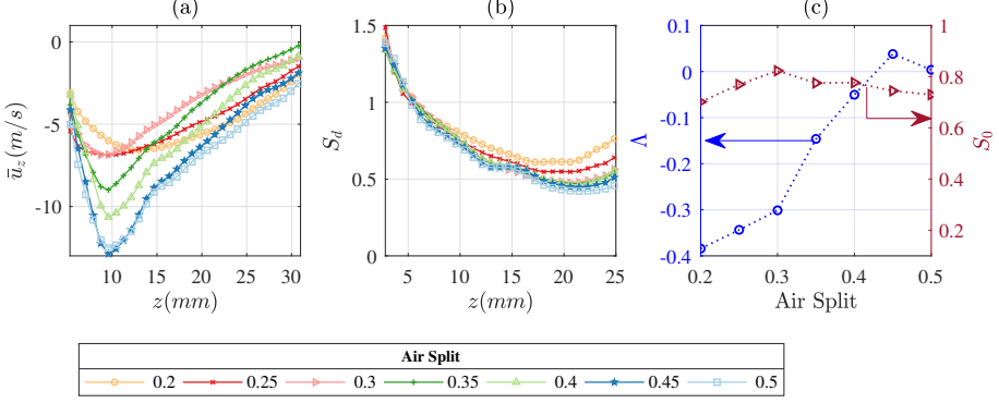
FIGURE 9. (a) Centerline time-averaged axial velocity, (b) swirl number, and (c) backflow ratio and swirl number at the downstream location of minimum mean centerline axial velocity for all air split conditions.
