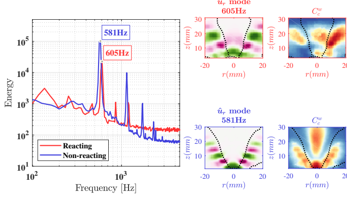
FIGURE 17. Transverse velocity mode shapes of the first SPOD mode and the weighted closeness centrality fields for both reacting (red) and non-reacting conditions (blue) conditions at the air split of 0.4. The black dotted line represents the limits of the recirculation zone ( \bar{u}_z = 0 )
