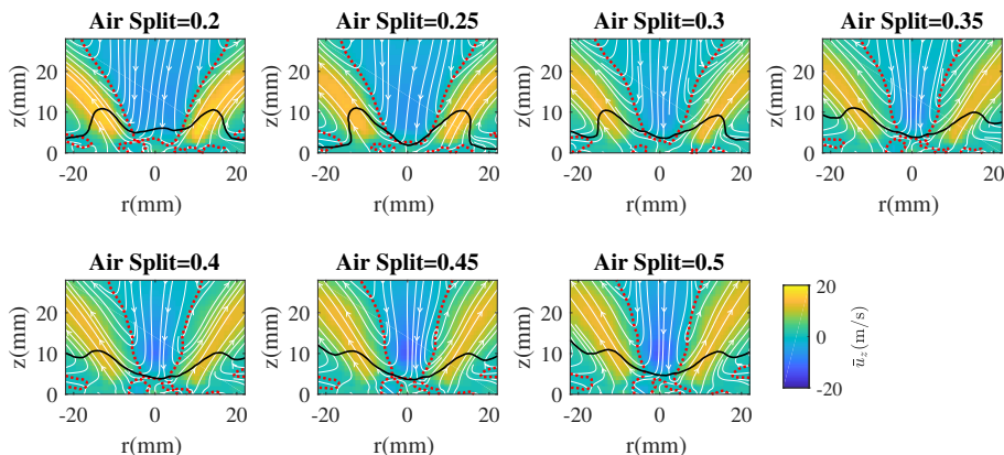
FIGURE 8. Time-averaged streamwise velocity component with streamlines (white solid lines) with the mean flame location ( \bar{c} = 0.5 ) depicted by the solid black lines and the limits of recirculation zone ( \bar{u}_z = 0 ) depicted as dotted red lines.
