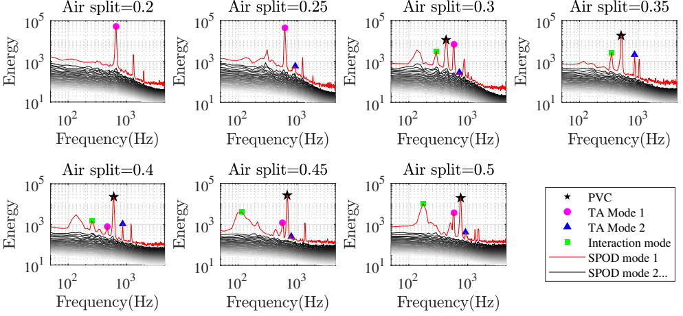
FIGURE 11. Modal spectra of velocity field obtained from spectral POD at all air splits for the reacting conditions.
