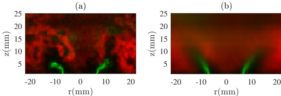
FIGURE 2. (a) Instantaneous and (b) time-averaged images of superimposed OH-PLIF (red contour) and acetone-PLIF (green contour) signals.
