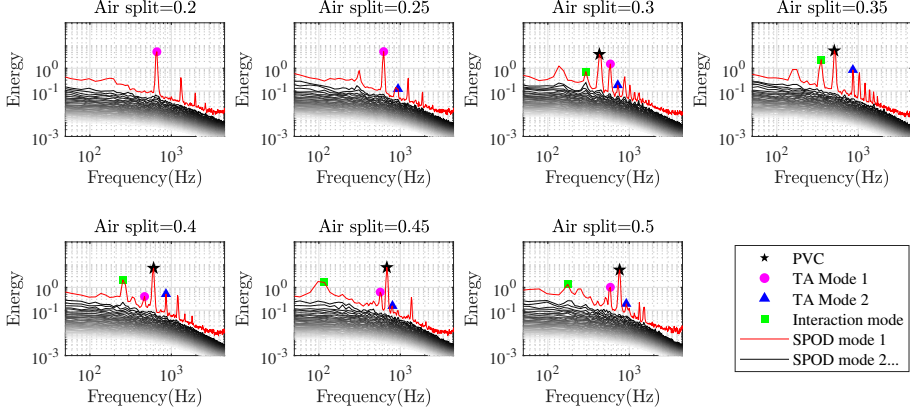
FIGURE 15. Modal energy spectra obtained from spectral POD on the composite velocity and OH-PLIF field.
