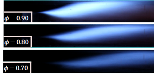
Fig. 8: Flame stabilized in a backwards-facing step combustor at three equivalence ratios [113]; reprinted with permission from S. Hong.
