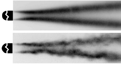
Fig. 6: Time-averaged (a) and instantaneous (b) images of a bluff-body stabilized flames on a ballistic bluff body [111]; reprinted with permission from B. Emerson.
