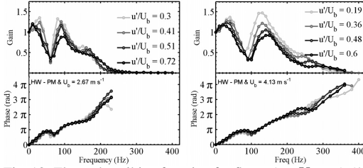
Fig. 18: Flame describing function for flame A at U_b = 2.67 m/s (left) and flame B U_b = 4.13 m/s (right) from Palies et al. [72]; reprinted with permission from Elsevier.
