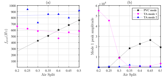
Fig. 24: Thermoacoustic and PVC mode frequency (a) and amplitude (b) as a function of air split in a dual-passage swirler [213].
