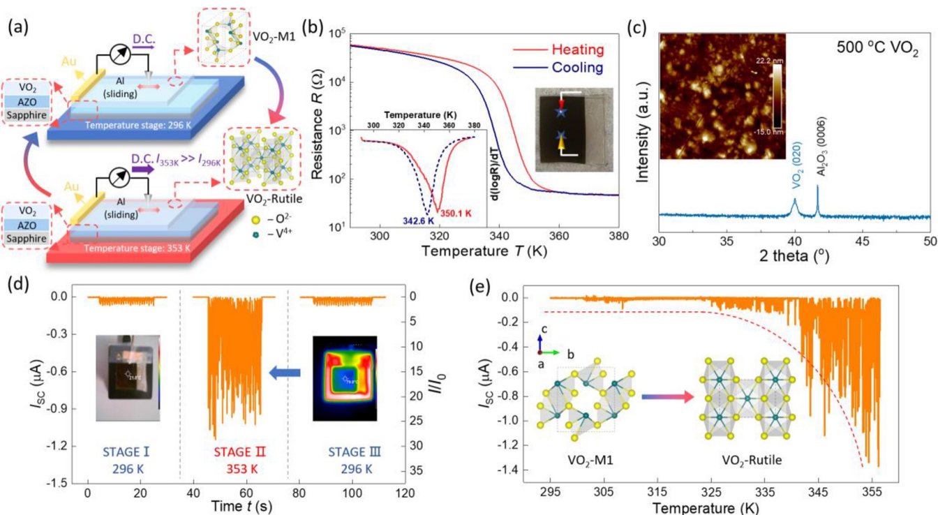
Figure 1. (a) Schematic illustration of Al/ \text{VO}_2 sliding contacts. (b) Resistance–temperature plots of the as-synthesized \text{VO}_2 thin film. The T_c value of \text{VO}_2 is around 345 K. Inset: resistivity change rate of \text{VO}_2 films. (c) XRD \theta – 2\theta spectra of \text{VO}_2 thin films on c-cut sapphire substrates. Inset: AFM topological image of the \text{VO}_2 thin film. (d) Short-circuit current ( I_{\text{sc}} ) at stage I before heating (room temperature: 296 K), at stage II on heating to 353 K, and stage III on cooling back to room temperature (296 K) under 0.1 MPa pressure. Inset: thermal image at stages I and III (left) and at stage II (right). (e) Real-time I_{\text{sc}} of Al/ \text{VO}_2 sliding contacts as the temperature is increased continuously under 0.1 MPa pressure. Inset: illustration of the crystal structure changing from \text{VO}_2 -M1 (monoclinic) to \text{VO}_2 -rutile (tetragonal).
