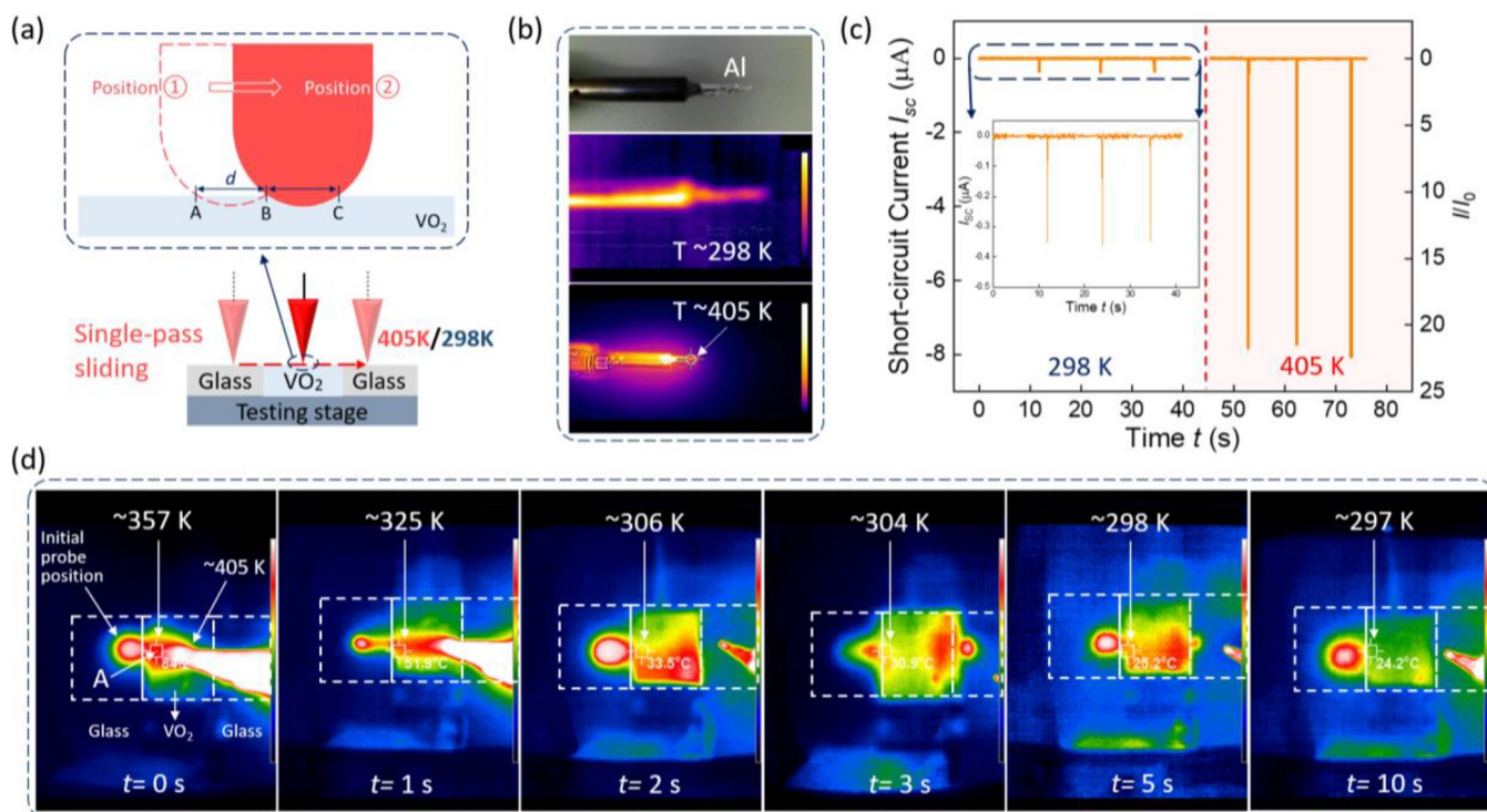
Figure 4. (a) Schematic demonstration of the tribovoltaic effect under fast a MIT transition with dynamic heating of \text{VO}_2 , where the \text{VO}_2 thin film sample is positioned between two glass slides and an Al-wrapped soldering probe is employed to perform sliding at both room temperature ( 298 \text{ K} ) and high temperature ( \sim 405 \text{ K} ). (b) Photo image (top) and IR images (middle, room temperature, 298 \text{ K} ; bottom, high temperature, \sim 405 \text{ K} ) of the probe. (c) Corresponding I_{\text{sc}} measurements at room temperature and high temperature with multiple testing cycles. The time interval between each cycles is 10 s. (d) Real-time IR images with local temperature distribution throughout a single-pass sliding process, from presliding to 10 s after sliding.
