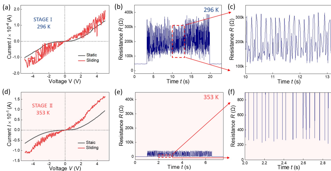
Figure 3. (a) Comparison of room-temperature I - V characterization of the Al/ \text{VO}_2 contact under static and sliding conditions. (pressure of 0.1 MPa, sliding speed of 15 \text{ mm s}^{-1} ). (b) Contact resistance fluctuation with Al/ \text{VO}_2 sliding contacts at room temperature ( \sim 296 \text{ K} ). (c) Enlarged figure showing the detailed contact resistance profile. (d) Comparison of I - V characterization of the Al/ \text{VO}_2 junction under static and sliding conditions (pressure of 0.1 MPa). (e) Resistance fluctuation with Al/ \text{VO}_2 sliding contacts after a phase transition ( \sim 353 \text{ K} ). (f) Enlarged figure showing the detailed contact resistance profile.
