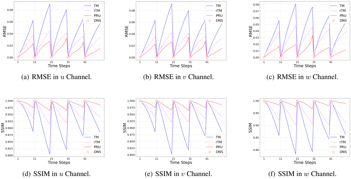
Figure 5: Change of RMSE/SSIM values produced by different DNS prediction models from the 1st to 50th time steps in a testing period with true DNS data for 10 time steps. (a)-(c) show the changes of RMSE values, and (d)-(f) show the changes of SSIM values for ( u, v, w ) three different channels.
