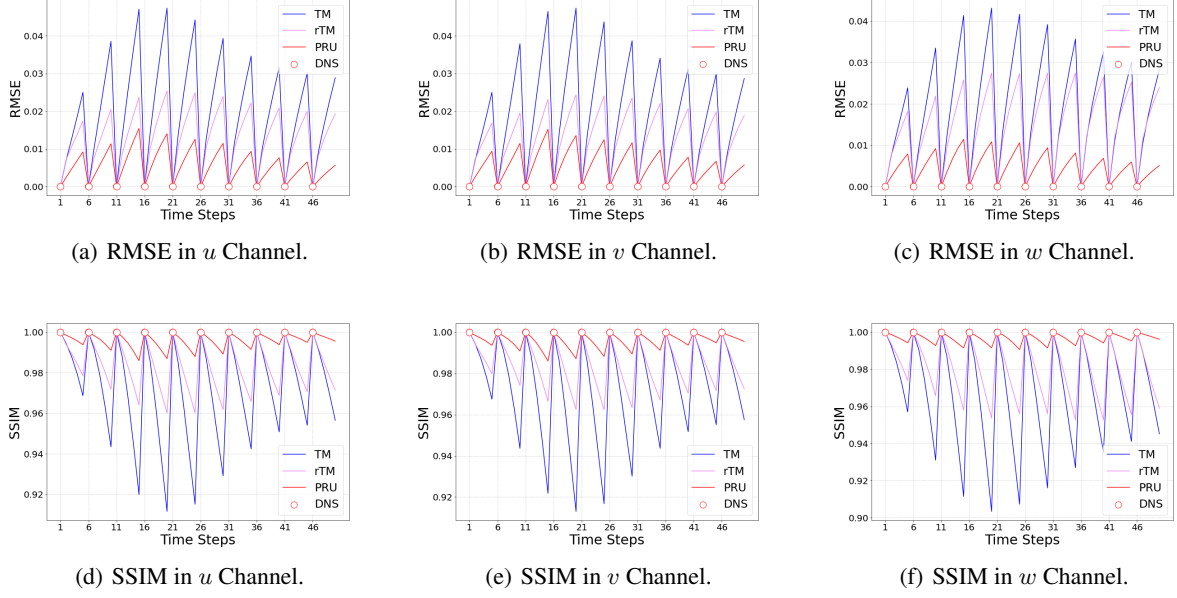
Figure 4: Change of RMSE/SSIM values produced by different DNS prediction models from the 1st to 50th time steps in a testing period with true DNS data for 5 time steps. (a)-(c) show the changes of RMSE values, and (d)-(f) show the changes of SSIM values for ( u, v, w ) three different channels.
