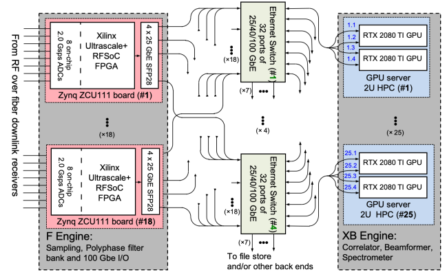
Figure 4. Signal processing is distributed over two stages. Antenna voltage signals are digitized and channelized in the first stage by 18 ZCU111 RFSoc boards. These data products are transported over 100 GbE for beamforming by a cluster of 25 HPCs each with two NVIDIA GPUs.
