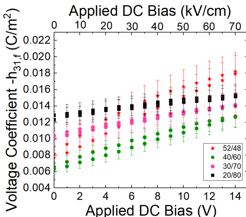
Figure 6. Voltage coefficient versus DC bias for various PZT compositions.
