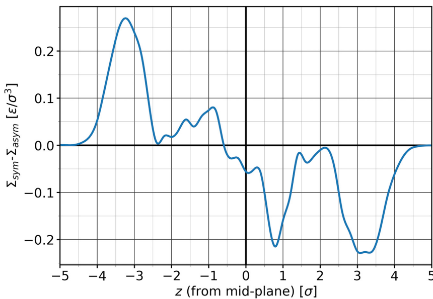
FIGURE 4 Difference between the lateral stress profiles of a completely symmetric membrane and an asymmetric membrane with \delta\ell = 2\% , as a function of the distance from the mid-plane. Neither membrane contains any cholesterol. To see this figure in color, go online.
