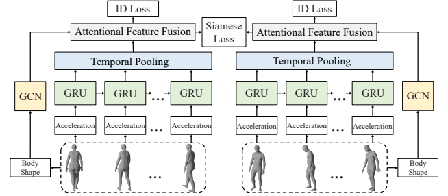
Figure 4: The person Re-ID model.
