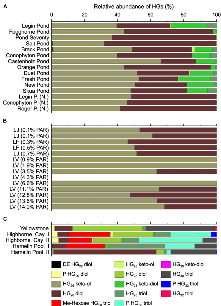
FIGURE 6 | Heterocyte glycolipid distribution in the meltwater ponds from the McMurdo Ice Shelf (A) . Samples with (N.) indicate ‘Nostoc spheres,’ which were collected in three different meltwater ponds. Panel (B) shows the results from the three different Antarctic lakes: Lake Joyce (LJ), Lake Fryxell (LF) and Lake Vanda (LV). The brackets show the percentage of photosynthetically active radiation (PAR) that reached the microbial mats. The PAR was adopted from previous studies (Jungblut et al., 2016; Mackey et al., 2017b, 2018; Matys et al., 2019). HGs in LV 4.3% PAR were below detection limit. Panel (C) shows the relative abundance of HGs in the microbial mats from the Yellowstone National Park (United States), Highborne Cay (Bahamas), and Hamelin Pool (Australia). DE, deoxyhexose; P, pentose; Me-hexose, methyl-hexose.
