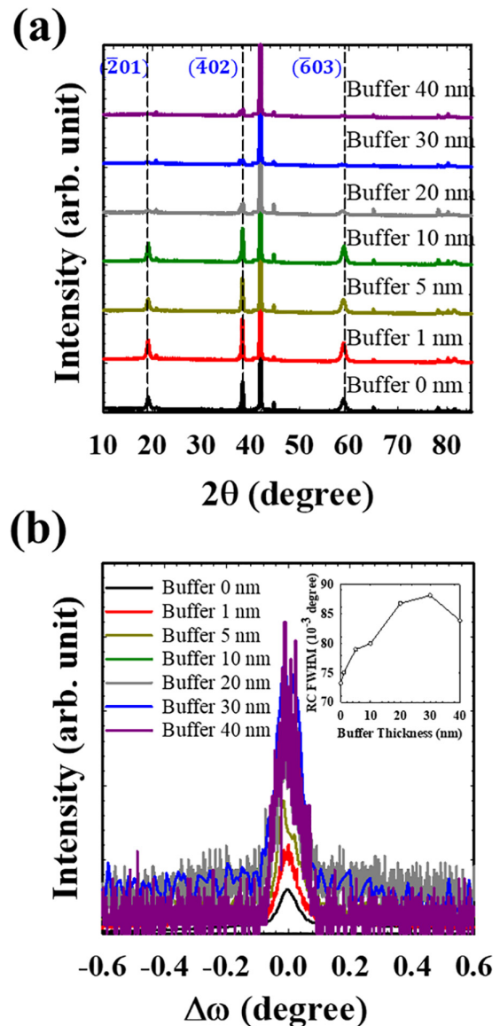
FIG. 2. (a) XRD pattern in \theta/2\theta scan mode showing that all \text{MgGaO} samples are \beta -phase with (201) orientation. (b) XRD rocking curves of (\text{Mg}_{0.074}\text{Ga}_{0.926})_2\text{O}_3 samples (402) peak and FWHM fitted with Gaussian method are plotted in the inset graph.
