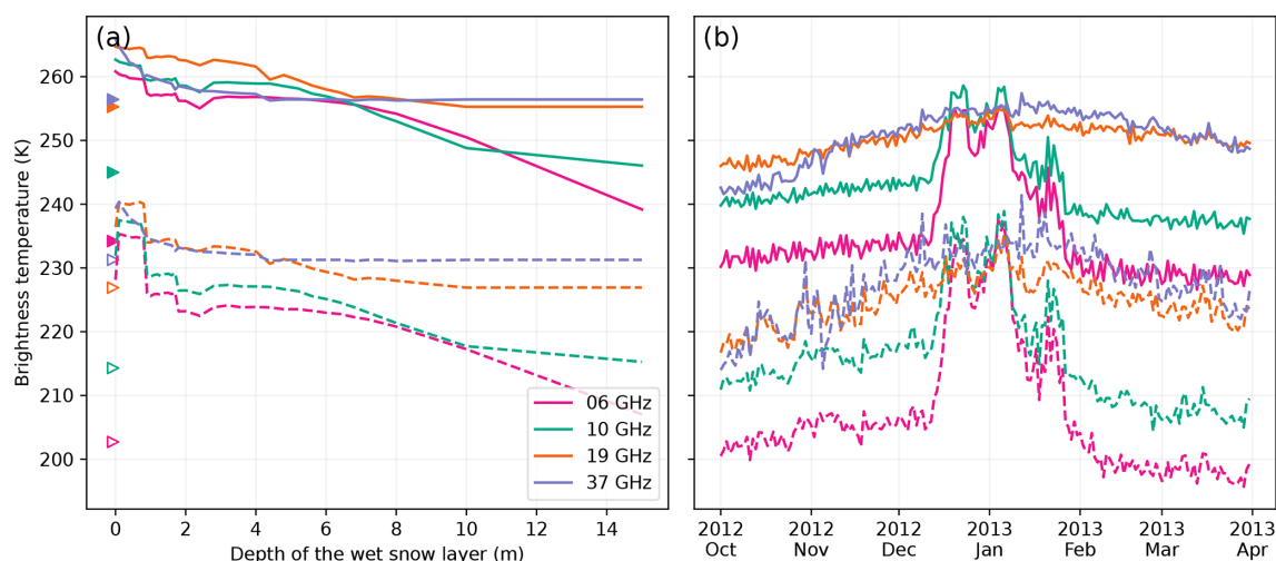
Figure 14. Brightness temperature as a function of the depth of the 10 cm thick wet snow layer at Halvfarryggen at V-pol (solid curves) and H-pol (dashed curves) (a). Values of dry brightness temperatures are marked by triangles. Each curve is the average of the 1000 best snowpacks. Time series of brightness temperature observations at Halvfarryggen (b).
