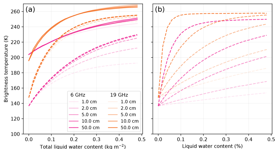
Figure 10. Brightness temperature as a function of the total liquid water content ( a ) and the volumetric liquid water content ( b ) for various wet snow layer thickness, for Roi Baudouin at 6 GHz (pink) and 19 GHz (orange), at V-pol (solid curves) and H-pol (dashed curves). V-pol is not on panel ( b ) for the sake of readability.
