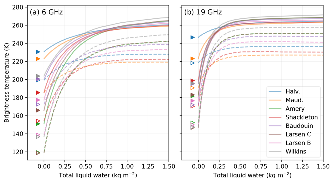
Figure 8. Brightness temperatures as a function of the liquid water content for all sites at V-pol (solid curves) and H-pol (dashed curves) at 6 GHz (a) and 19 GHz (b). The values of the dry brightness temperatures are marked by the triangles.
