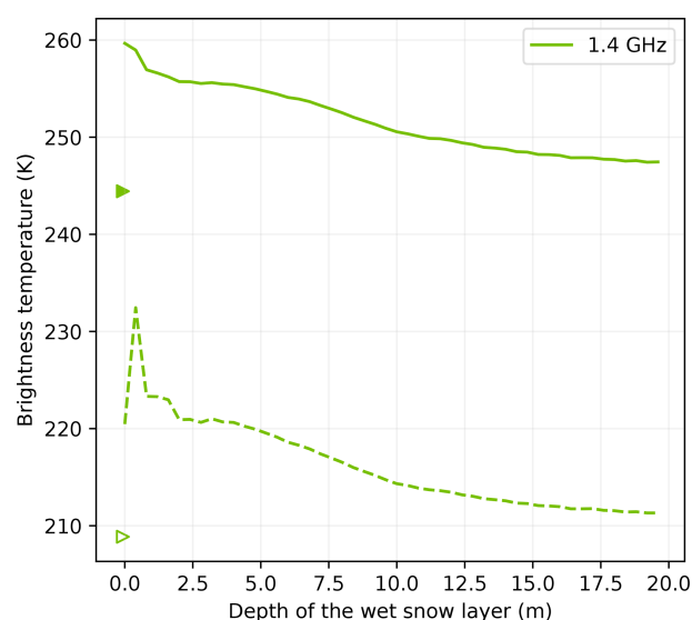
Figure 18. Brightness temperature at Roi Baudouin as a function of the depth of the 30 cm thick wet snow layer at the L band at V-pol (solid) and H-pol (dashed). The simulated dry brightness temperatures are marked by the triangles.
