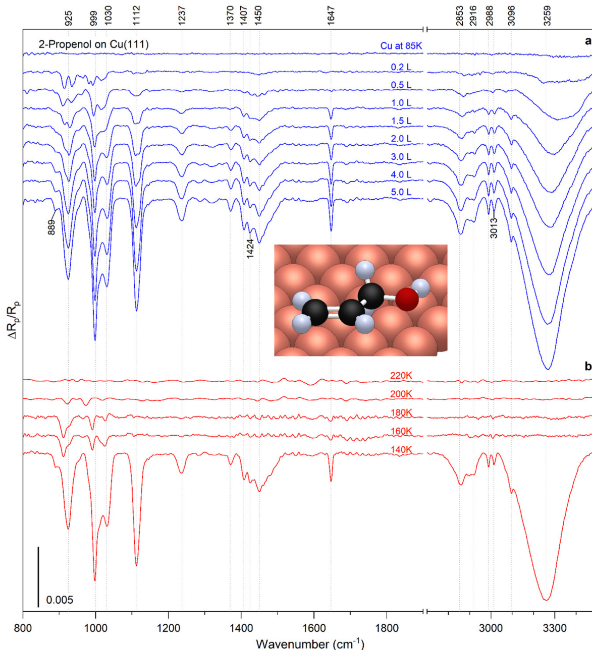
Fig. 5 (a) RAIR spectra (blue) of 2-propenol on Cu(111) at 85 K versus exposures. (b) RAIR spectra (red) after the Cu(111) surface at 85 K was exposed to 5 L of propenol, annealed to the indicated temperatures for 1 minute, then cooled back to 85 K where the spectra were acquired. The inset shows the structure of monolayer 2-propenol on Cu(111).
