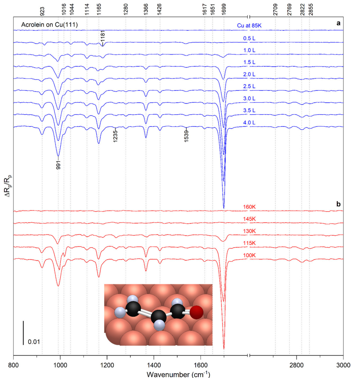
Fig. 1 (a) RAIR spectra (blue) of acrolein on Cu(111) at 85 K versus exposures. (b) RAIR spectra (red) after the Cu(111) surface at 85 K was exposed to 4 L of acrolein, annealed to the indicated temperatures for 1 minute, then cooled back to 85 K where the spectra were acquired. The inset shows the structure of monolayer acrolein on Cu(111).
