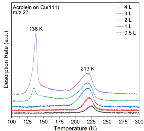
Fig. 2 TPD spectra of acrolein adsorbed on Cu(111) with increasing exposure.
