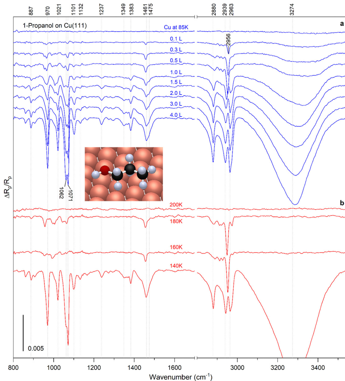
Fig. 7 (a) RAIR spectra (blue) of 1-propanol on Cu(111) at 85 K versus exposures. (b) RAIR spectra (red) after the Cu(111) surface at 85 K was exposed to 4 L of propanol, annealed to the indicated temperatures for 1 minute, then cooled back to 85 K where the spectra were acquired. The inset shows the structure of monolayer 1-propanol on Cu(111).
