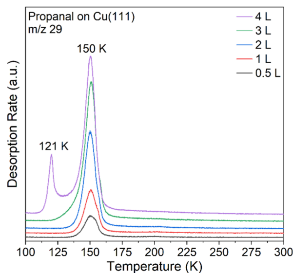
Fig. 4 TPD spectra of propanal adsorbed on Cu(111) at 85 K with increasing exposure.
