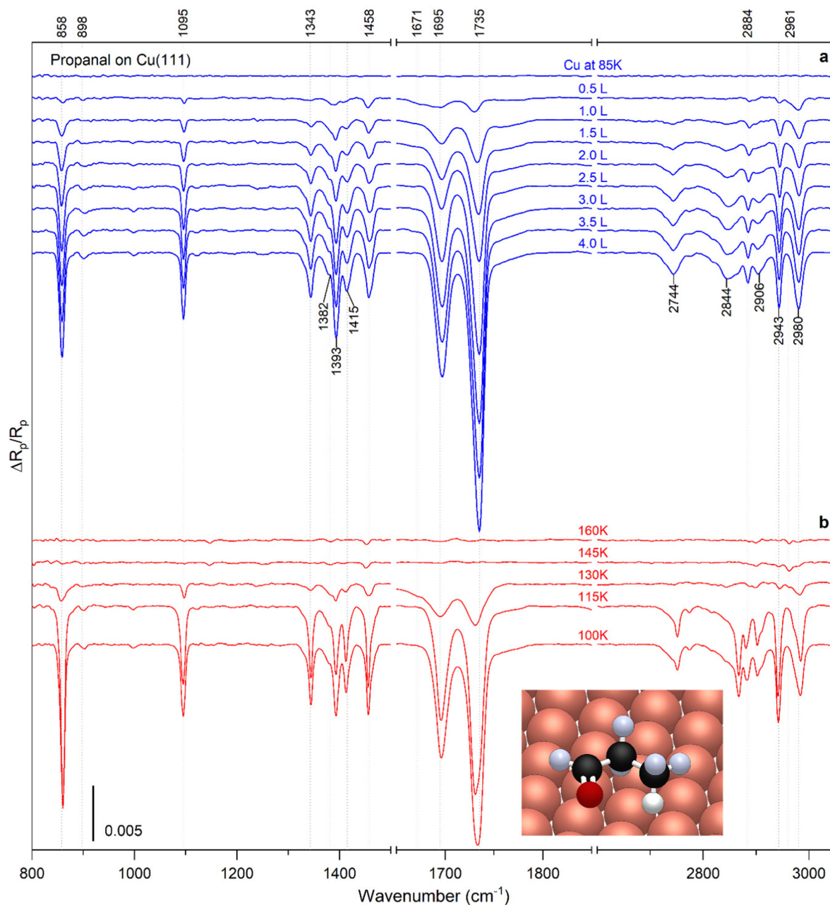
Fig. 3 (a) RAIR spectra (blue) of propanal on Cu(111) at 85 K versus exposures. (b) RAIR spectra (red) after the Cu(111) surface at 85 K was exposed to 4 L of propanal, annealed to the indicated temperatures for 1 minute, then cooled back to 85 K where the spectra were acquired. The inset shows the structure of monolayer propanal on Cu(111).
