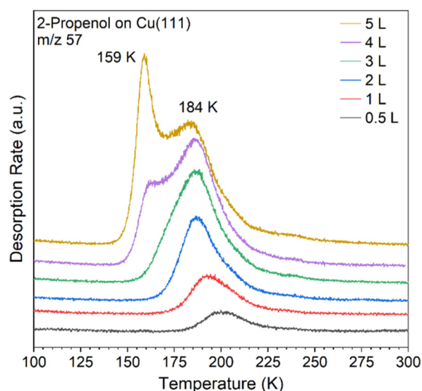
Fig. 6 TPD spectra of 2-propenol adsorbed on Cu(111) at 85 K with increasing exposure.
