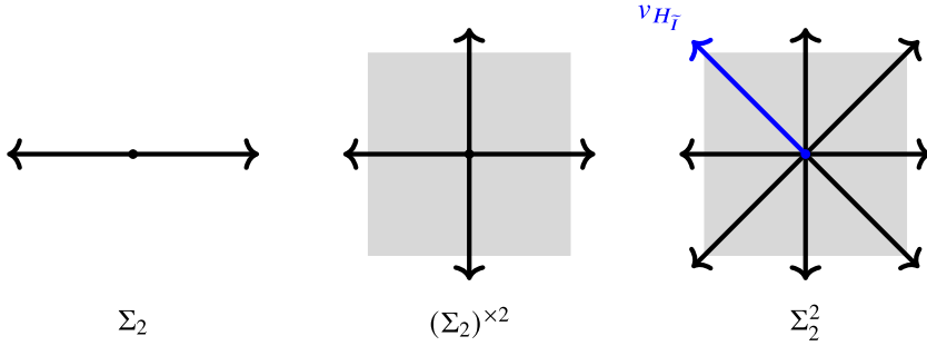
Figure 5. The fan \Sigma_2^2 , obtained via stellar subdivision from the Cartesian product of two copies of the fan \Sigma_2 . The labeled vector v_{H_I} corresponds to the nested set \tilde{\mathbf{I}} = (\{1, 2\}, \mathbf{a}) in which \mathbf{a}(1) = 1 and \mathbf{a}(2) = 0 .
