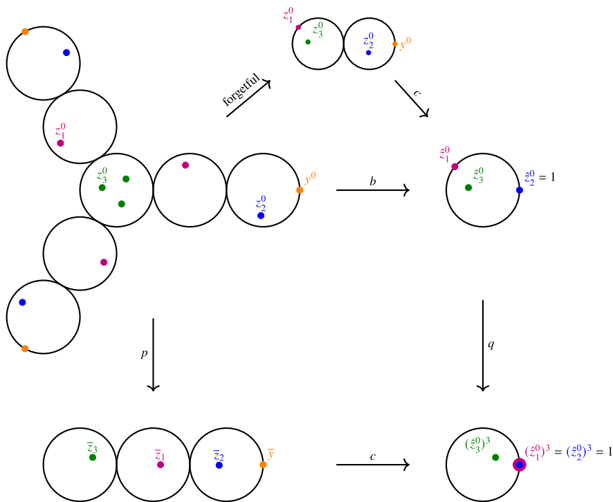
Figure 3. A representation of the maps in diagram (7) in the case where r = n = 3 , with the points x^\pm omitted for clarity. In the upper-right corner, the three coordinates in (\mathbb{P}^1)^3 are \zeta , 1 and a point z_3^0 that is not a third root of unity. In the lower-right, the three coordinates are 1, 1 and (z_3^0)^r .
