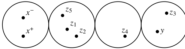
Figure 2. A point of \overline{\mathcal{M}}_6^1 .
