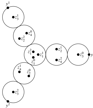
Figure 1. A stable (3,4) -curve, where each circle represents a \mathbb{P}^1 component and \sigma is the rotational automorphism. Not pictured are the marked points x^+ and x^- , which are the two fixed points of \sigma and must both lie on the central component.
