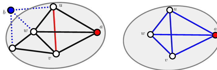
Figure 9. Remove from C the edges from b (blue dotted) and add red edge e . Circuit B (blue).
