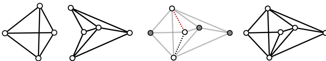
Figure 5. A complete K_4 graph, a 4-wheel W_4 , their common edges (dotted, with elimination edge in red), and their combinatorial resultant, which has more than 2n - 2 edges and thus is not a circuit.
