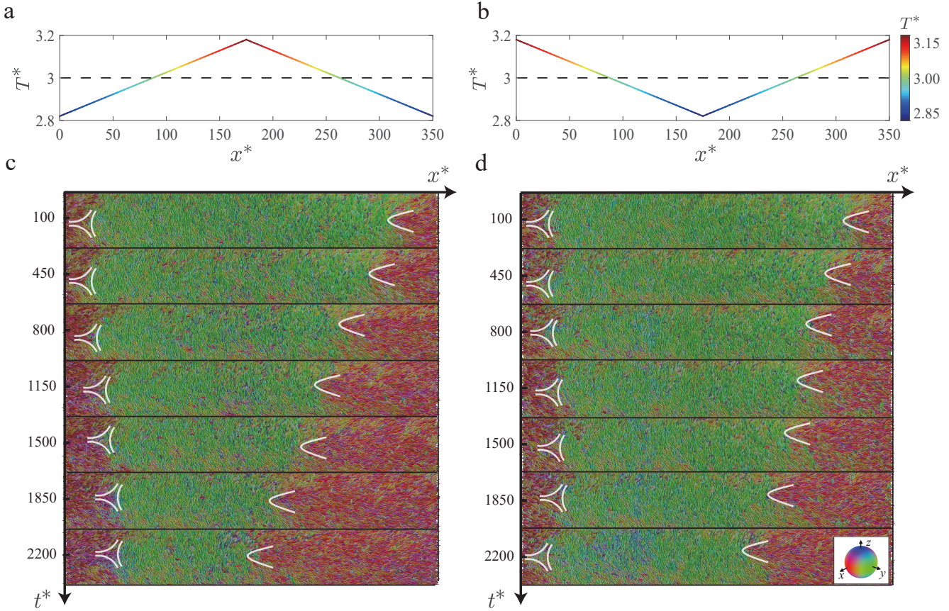
Fig. 6 Temperature gradient effect for defect motion. Diagram of temperature distribution along the x -axis of positive (a) and negative (b) temperature gradient. Spatiotemporal kimograph of defects motion for positive (c) and negative (d) gradient scenario. The color bar in (b) indicates the temperature magnitude. Inset in (d): colormap indicates the particle orientation.
